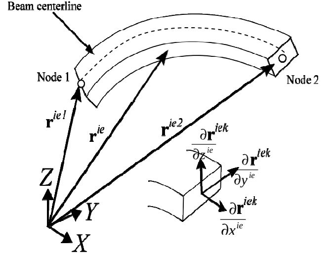
Figure 1: ANCF Beam Element Coordinates
