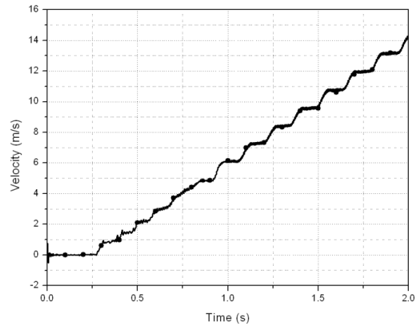
Figure 5: X velocity of the center of mass of the chassis
