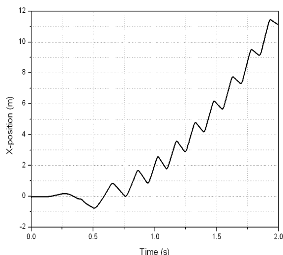
Figure 6: X coordinate of the position vector of a point on the rubber chain
