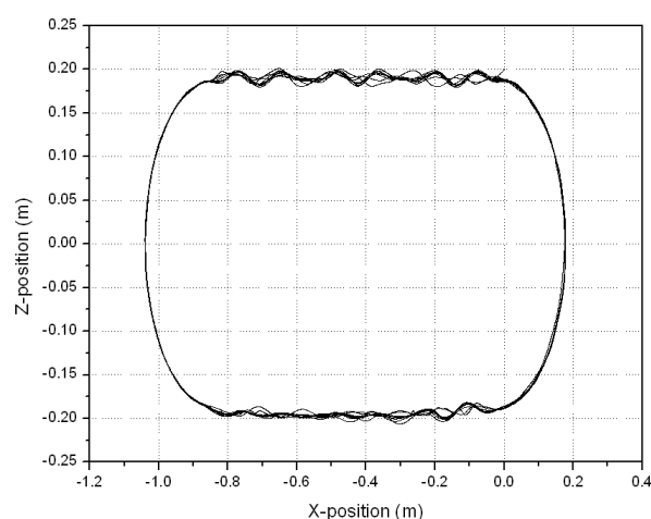
Figure 8: Trajectory of the position vector of a point on the rubber chain
