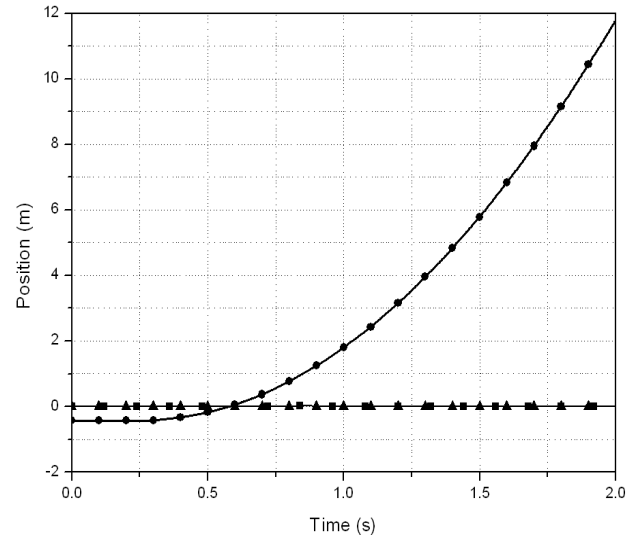
Figure 4: Position of Center of Mass of the Chassis (—●— X coordinate; —■— Y coordinate; —▲— Z coordinate)
