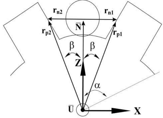
Figure 2: Geometry of contact between rigid sprocket teeth and the C^0/C^1 chain
