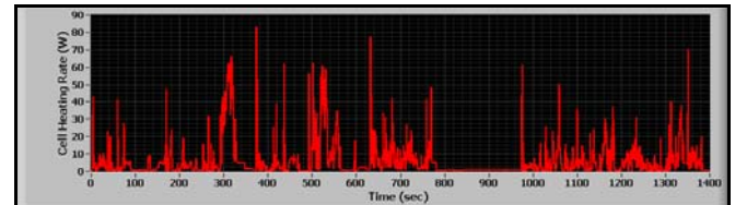
Figure 17: Off-Road Driving Profile #1 Battery Cell Heating Rate
