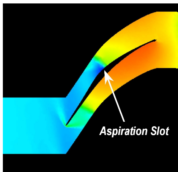
Fig. 3 Computed blade flowfield with aspiration
