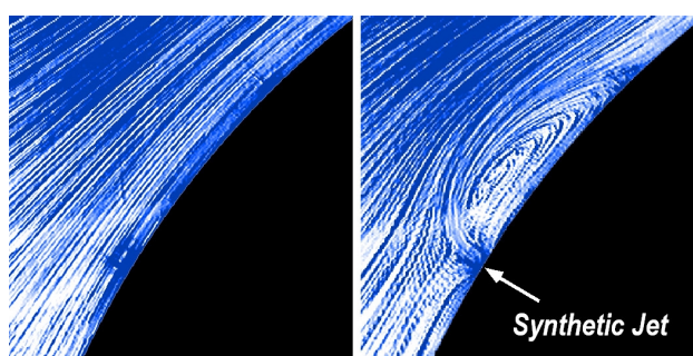
Fig. 8 Trapped vortex induced by synthetic jet
