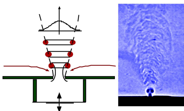
Fig. 7 Synthetic jet schematic and schlieren visualization
