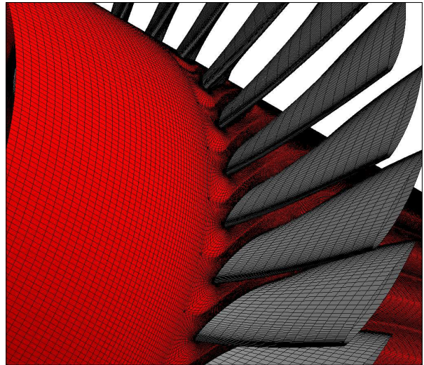
Figure 2.4: Rotor blade zoom (single row system).
