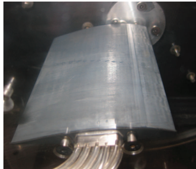
(b) Blade installed on cylinder in wind tunnel
