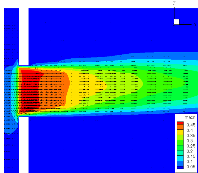
Figure 2.16: Single exit jet Mach contours.
