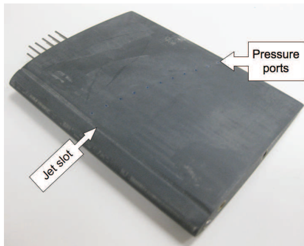
(a) Jet slot and pressure ports locations
