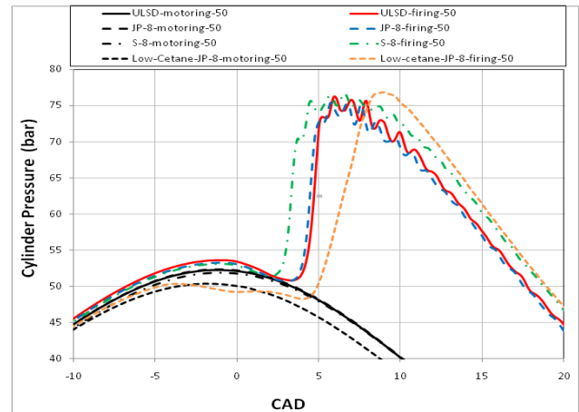
Figure 4.a: Cylinder gas pressure for different fuels at inlet air temperature of 50 °C and IMEP of 3 bar (Speed = 1500 rpm, Inj. Pressure = 800 bar, SOI = -2.0 CAD, SOI for JP-8#31 = -6.0 CAD)
