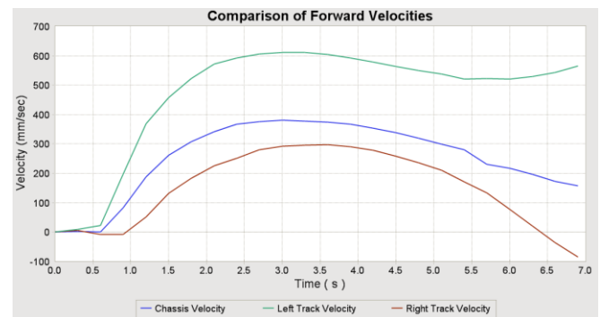
Figure 15. Comparison of the Forward Velocities of the Vehicle Chassis and the Left and Right Tracks.
