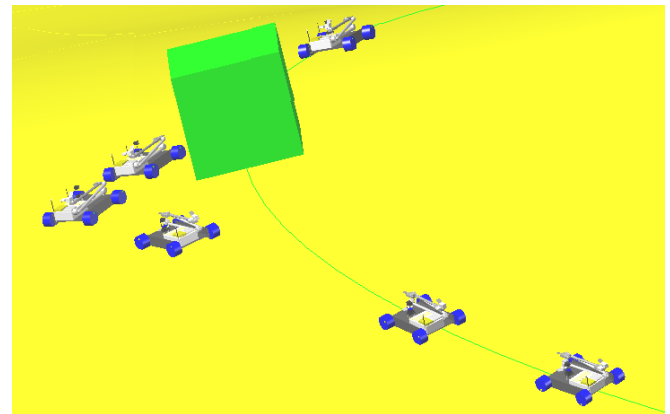
Figure 10. Robot motion around the obstacle in an autonomous avoidance maneuver.
