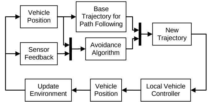
Figure 8. Path Planning and Avoidance Schematic
