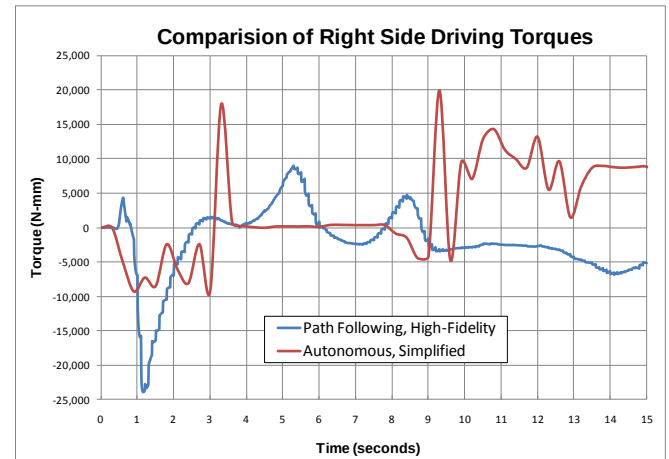
Figure 14. Right Side Driving Torques
