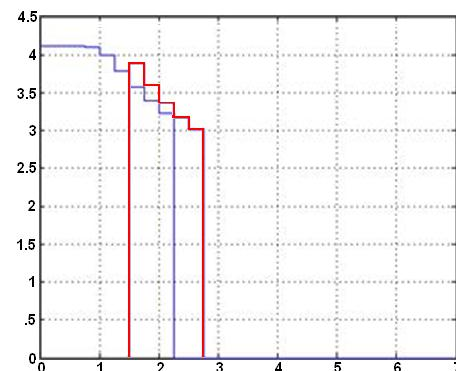
Figure 11. Sensor readings at 0 (red) and -10 (blue) degrees (distance to the obstacle) vs. simulation time
