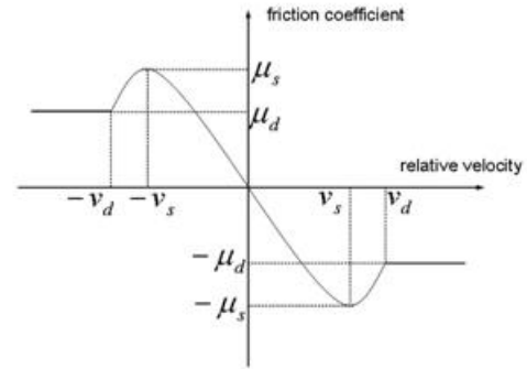
Figure 6. Friction Coefficient as a Function of Velocity.
