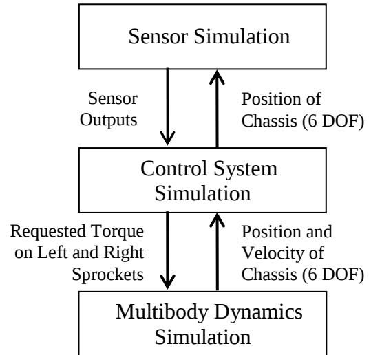
Figure 1. Software Architecture.
