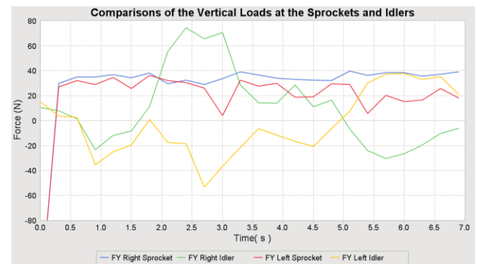
Figure 16. Vertical loads at the Sprockets and Idlers
