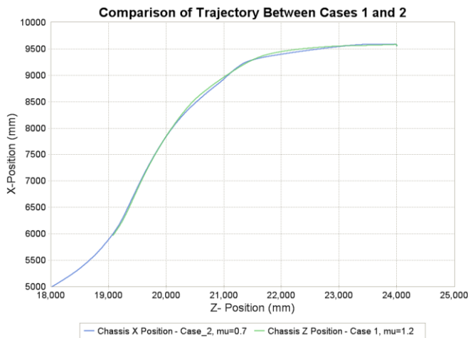
Figure 13. Comparison of the trajectory followed by the chassis of the tracked vehicle for the two cases.
