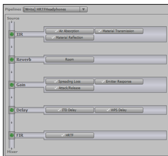
Figure 2: Modular propagation pipeline
