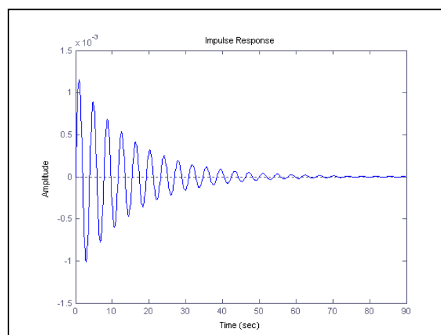
Figure 5: Impulse Response Function – Time Domain
