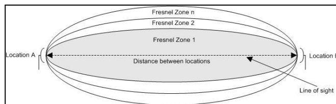
Figure 12: Fresnel Zone Shapes
