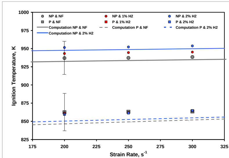
Fig. 4 \text{H}_2 counterflow diffusion flame ignition temperatures as a function of strain rate for air and ultra-lean \text{H}_2 pre-mixtures as the oxidizer with and without MGA plasma activation.
