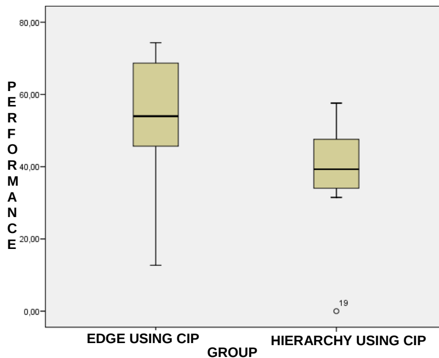
Figure N° 10. Boxplot of Performance variable Hypothesis D.
