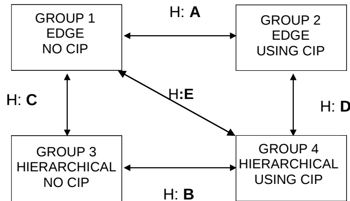
Figure N°6. Groups and hypotheses.
