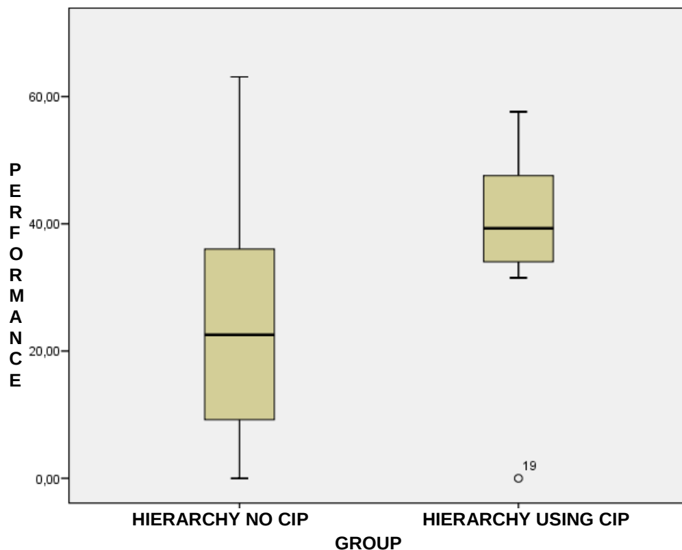
Figure N° 8. Boxplot of Performance variable Hypothesis B (H-B).
