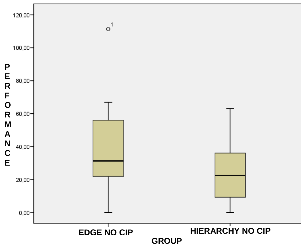
Figure N° 9. Boxplot of Performance variable Hypothesis C.
