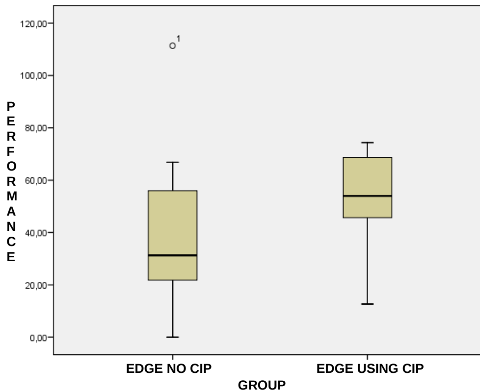
Figure N° 7. Boxplot of Performance variable, H-A.
