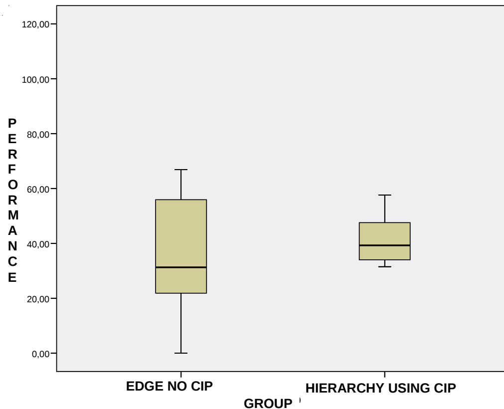
Figure N° 11. Boxplot of Performance variable.
