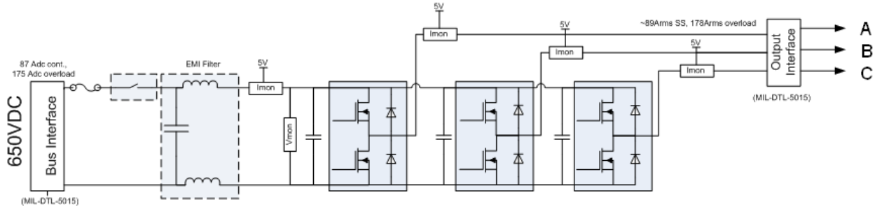
Figure 5. Motor Driver Inverter Schematic.
