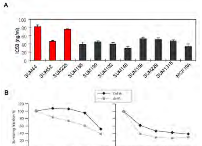
Figure 3. (A) IC 50 values for the Tunicamycin (Tm), in ten breast cancer cell lines as well as nontransformed human mammary epithelial cell line MCF10A (B) Cell viability of ERLIN2 knockdown and control SUM-225 cells was measured with MTT assays after exposure to different concentrations of the Tm or Tg for 72 hours.
