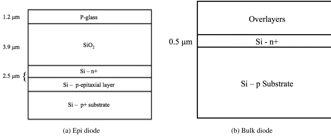
Figure III.1: Cross sections of the two bulk silicon diodes used in this work. The device shown in (a) was fabricated by Sandia National Laboratories in a 0.25 \mu\text{m} process. The device shown in (b) was fabricated in a 45 nm foundry process.
