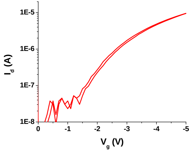
Figure 6: Transfer curve for a 50um pentacene on \text{ZrO}_2 device measured using a pulsed gate voltage.
