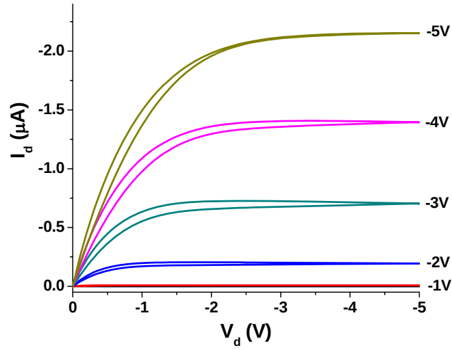
Figure 3: Output characteristics for a 50um channel length pentacene transistor on ZrO2.
