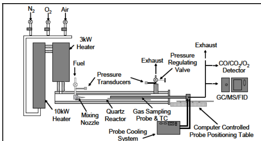
Figure 1. Pressurized Flow Reactor (PFR) schematic.
