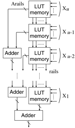
Figure 2. Architecture for NFG based on a monolithic EVMDD.
