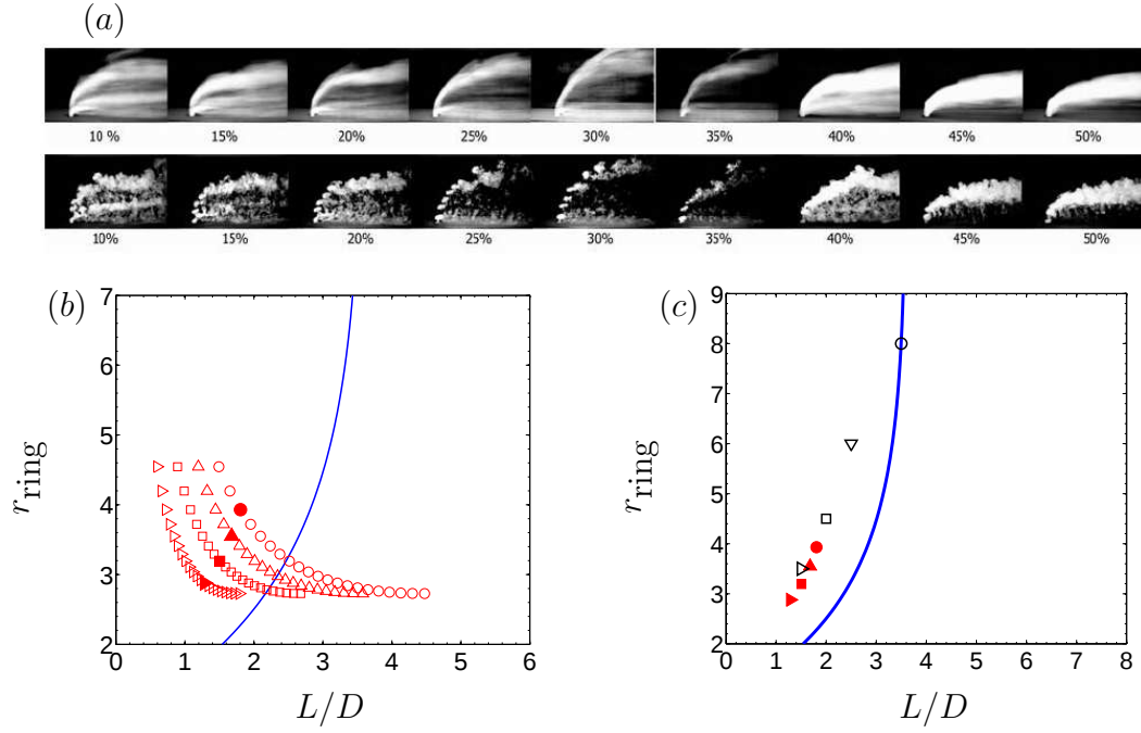
Figure 4.13: (a) Figure 4 from experiment of Shapiro et al. (2006), reprinted by permission; mean and instantaneous flow-field (case 1, U'_{j,\text{rms}} = 1.5 m/s) with forcing frequency f = 110 Hz for duty cycle ranging from 10% to 50%. Maximum jet penetration occurs at 30% duty cycle corresponds to optimal pulse width ( \tau = 3 ms). (b) The experimental conditions for varying pulse width or duty cycle are transformed in regime map for four frequencies: \circ , 44 Hz; \triangle , 55 Hz; \square , 73.5 Hz; \triangleright , 110 Hz. Filled symbols show the optimal conditions ( \tau = 3 ms) at corresponding frequencies. The solid line denotes the transition curve. (c) Optimal conditions from experiments are compared to simulations. Filled and open symbols correspond to experiment and simulations respectively.
