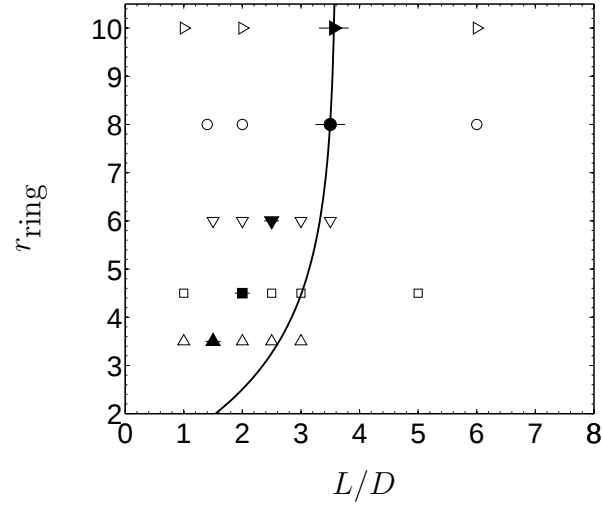
Figure 4.8: Simulation conditions are plotted in stroke ratio and ring velocity ratio coordinates. ○, case I & II; ▽, case III; □, case IV & V; △, case VI; ▷, case VII. The filled-symbols denote the optimal stroke ratio (table 4.1) at the corresponding ring velocity ratios. The solid curved line denotes the transition curve for a single vortex ring in crossflow. The horizontal bars around the optimal stroke ratios denote the uncertainty in each case.
