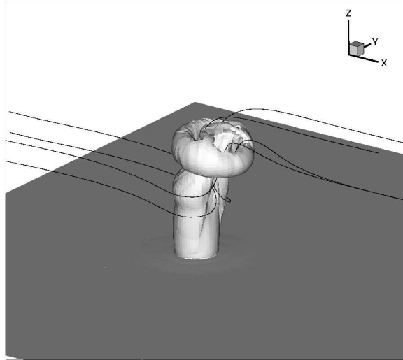
Figure 3.15: Iso-surfaces of vorticity along with some 3D streamlines for L/D = 6 and r = 6 . The stream lines show the downstream entrainment of the crossflow fluid.
