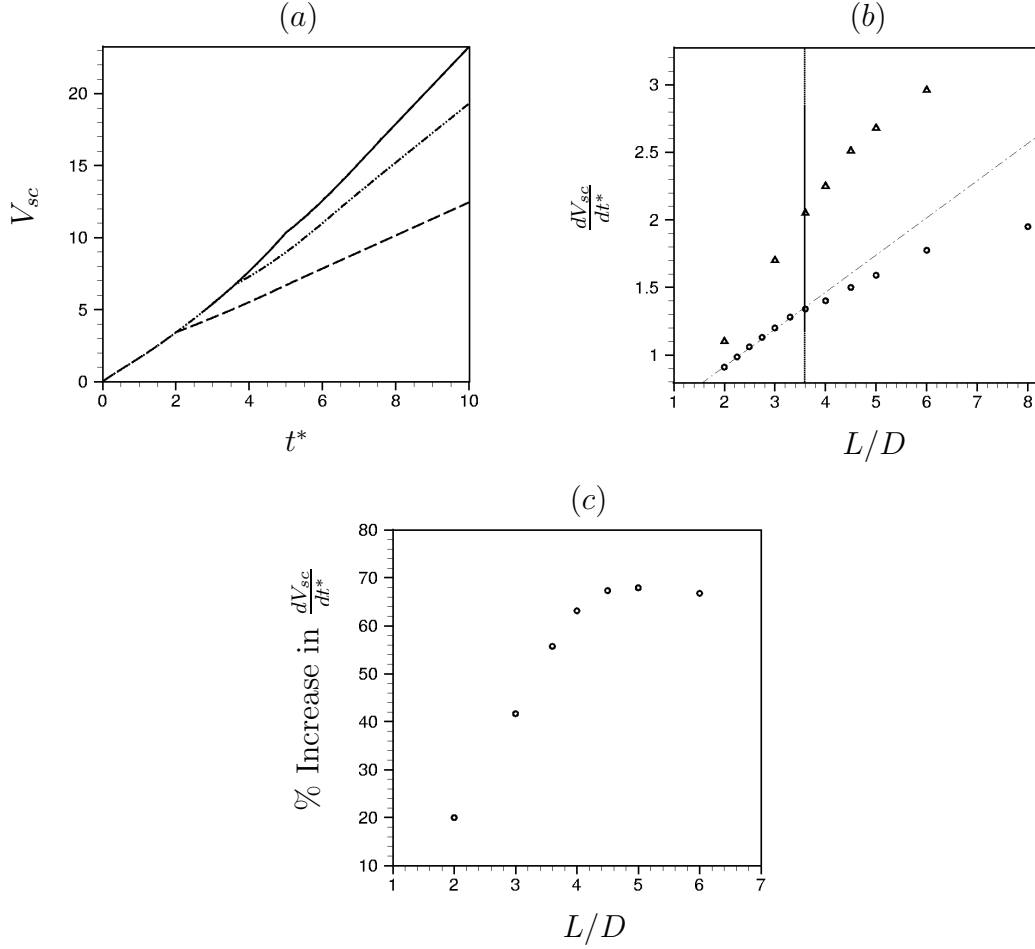
Figure 3.20: (a) Variation of volume of scalar-carrying fluid with time for different stroke ratios and r = 3 : --- , L/D = 2.0 ; -.-.- , L/D = 3.6 ; — , L/D = 5.0 . (b) The rate of change of scalar volume after formation against the stroke ratio for r = 3 : \Delta . The results for the vortex rings in the absence of crossflow are also shown: \circ . The vertical line denotes the formation number. (c) Percentage increase in the rates due to crossflow are plotted against the stroke ratio. Note that the percentage increment is maximum around L/D = 5 .
