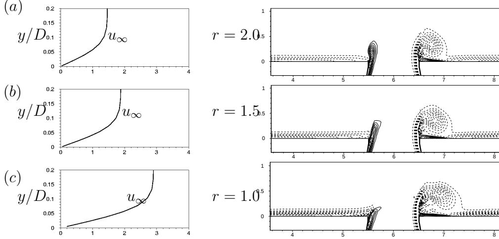
Figure 3.10: Low velocity ratio cases: (a) r = 2.0 , (b) r = 1.5 and (c) r = 1.0 . Crossflow boundary layer profiles and the vorticity contours in the symmetry plane are shown at t^* = 1.0 for each case. Note that the vorticity from the nozzle boundary layers is cancelled by opposing vorticity in the crossflow boundary layer at the upstream side of the nozzle exit.
