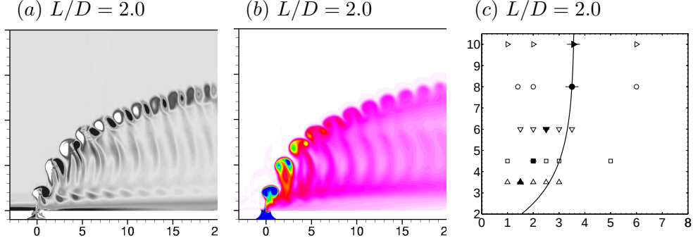
Figure 1.3: Low Reynolds number simulations of pulsed jet in crossflow. Contours of z vorticity (a) and scalar concentration (b) in symmetry plane. Ring velocity ratio, r_{\text{ring}} = 4.5 and duty cycle is at 20%. Optimal conditions are shown. (c) Optimal pulsing conditions from a number of simulations are plotted on the regime map.
