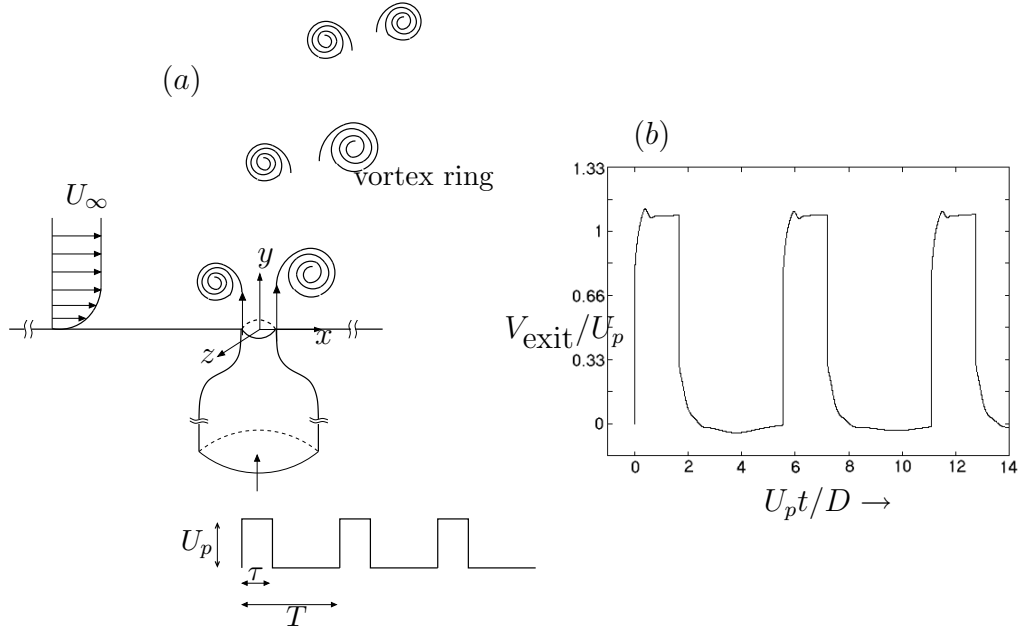
Figure 4.2: (a) A schematic of the problem. (b) Typical waveform at the nozzle exit resulting from a square waveform specified at the nozzle inflow.
