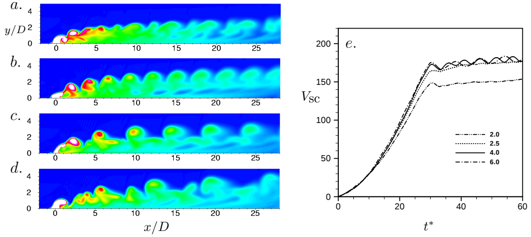
Figure 4.20: Ring velocity ratio = 1.0, duty cycle = 75%. Contours of scalar in the symmetry plane at different stroke ratios: (a) 2.0, (b) 2.5, (c) 4.0 and (d) 6.0. (e) Variation of total volume of scalar carrying fluid in the domain with time. Ring velocity ratio is 1.0, duty cycle is 75% and different stroke ratios are considered.
