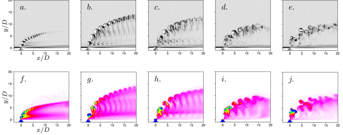
Figure 4.7: Case V: Contours of z vorticity (fig. a–e ) and scalar concentration (fig. f–j ) in symmetry plane. Ring velocity ratio, r_{\text{ring}} = 4.5 and duty cycle is 20% ( U_p = 3.0, U_\infty = 0.67 ). Strouhal number is varied: ( a ) & ( f ) St = 1.0 ; ( b ) & ( g ) St = 0.5 ; ( c ) & ( h ) St = 0.4 ; ( d ) & ( i ) St = 0.333 ; ( e ) & ( j ) St = 0.2 . Note that the optimal penetration is obtained at St = 0.5 .
