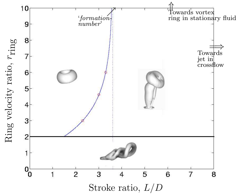
Figure 4.1: Regime map showing three different flow structures of vortex rings in crossflow (Sau & Mahesh 2008).
