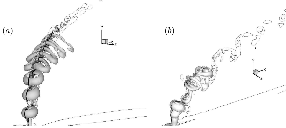
Figure 4.9: (a) Ring interactions. (b) Ring-column interactions.
