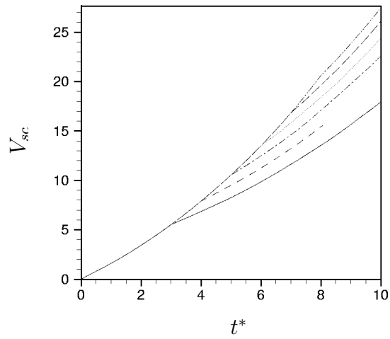
Figure 3.21: Variation of volume of scalar-carrying fluid with time for different stroke ratios and r = 1 : — , L/D = 3.0 ; ---- , L/D = 4.0 ; —·— , L/D = 5.0 ; ..... , L/D = 6.0 ; ---- , L/D = 7.0 ; -·-·- , L/D = 8.0 . Note that the slope of the volume curve after formation is almost the same for all stroke ratios.
