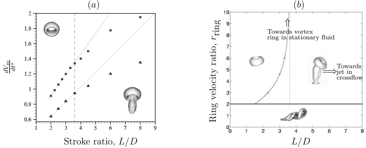
Figure 1.2: (a) Optimal entrainment by vortex rings in quiescent air. The dotted lines correspond to two different Schmidt numbers. Note the optimal stroke ratio – the ‘formation number’ separates two different physical regimes at both Schmidt numbers. (b) Vortex ring in crossflow. Regime map showing three regimes with different flow structure and entrainment characteristics.
