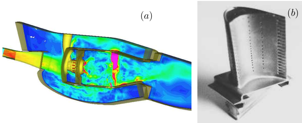
Figure 1.1: (a): Instantaneous snapshot of contours of velocity magnitude from simulations in a gas-turbine combustor (Mahesh et al. 2004). (b): Turbine blade with film-cooling holes visible.
