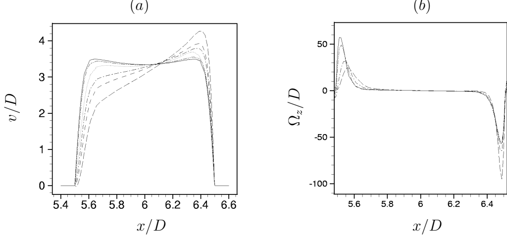
Figure 3.2: (a) v -velocity profiles at the nozzle exit in the symmetry plane at t^* = \overline{U}_{exit}t/D = 1.0 : —, without crossflow ( r = \infty ); —·—, r = 6 ; ·····, r = 3 ; — — —, r = 2.0 ; — — —, r = 1.5 ; — — —, r = 1.0 . (b) Corresponding span-wise vorticity, \Omega_z/D profiles: —, without crossflow ( r = \infty ); —·—, r = 6 ; —·—, r = 2.0 ; — — —, r = 1.0 .
