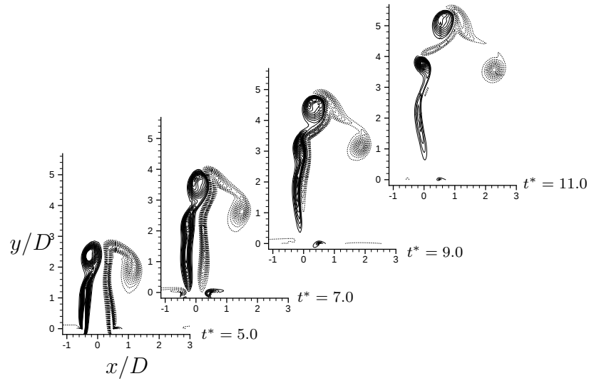
Figure 3.6: Vorticity contours in the symmetry plane for L/D = 6 and r = 6 at different time instants.
