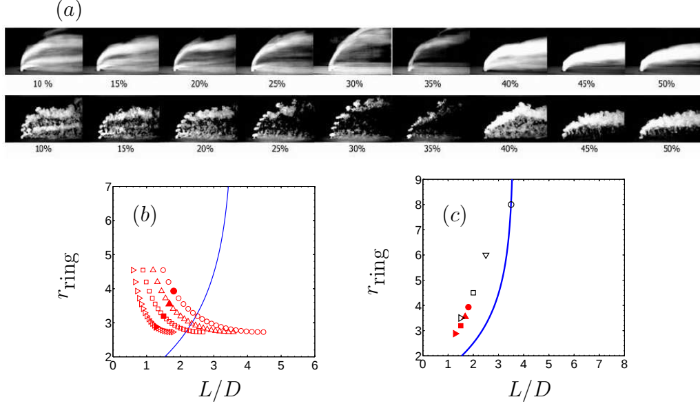
Figure 1.4: (a) Figure 4 from experiment of Shapiro et al. (2006), (case 1, U'_{j,\text{rms}} = 1.5 m/s) with forcing frequency f = 110 Hz for duty cycle ranging from 10% to 50%. Note maximum jet penetration occurs at 30% duty cycle and corresponds to optimal pulse width ( \tau = 3 ms). (b) The experimental conditions for varying pulse width or duty cycle are transformed onto regime map at four frequencies, where the filled symbols show the optimal conditions. (c) Optimal conditions from experiments (red) are compared along with simulations (black).
