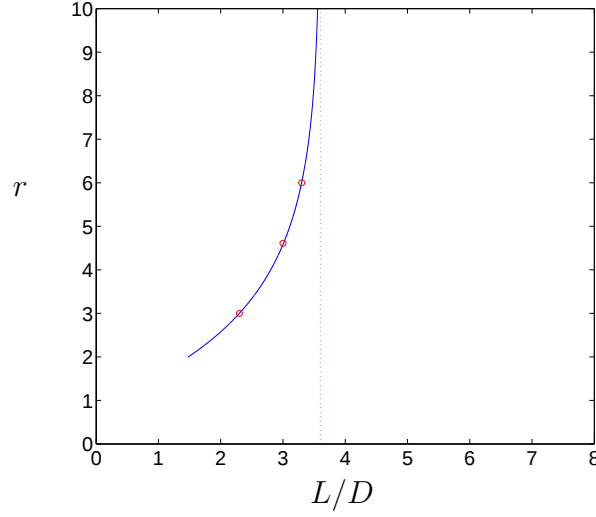
Figure 3.8: The transition curve separates two regimes of flow in the presence of crossflow. The dotted line represents the transition line in stationary flow.
