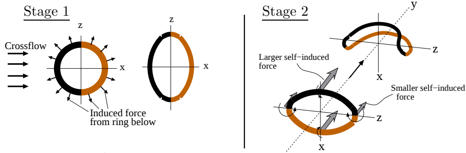
Figure 4.10: Schematic to explain ring deformation.
