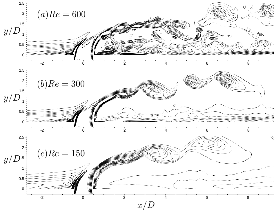
Figure 3.12: Vorticity contours in the symmetry plane at t^* = 20 for r = 1.0 and L/D = 100 . (a) Re = 600 , (b) Re = 300 , (c) Re = 150 . Note that shedding of the hairpin vortices is unstable at Re = 600 . The shedding is very periodic for lower Reynolds number.
