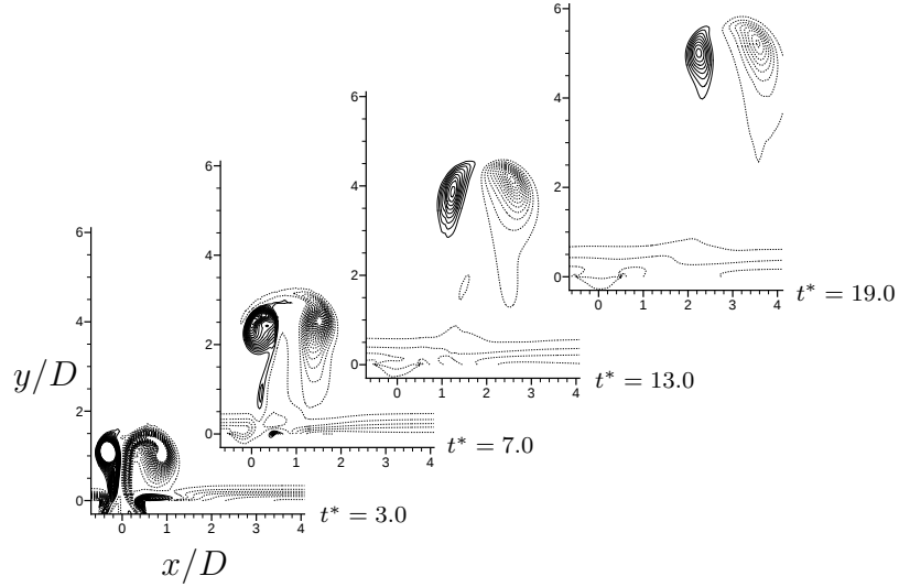
Figure 3.3: Vorticity contours for L/D = 2 and r = 6 at different time instants. The solid and dashed lines denote positive and negative values respectively.
