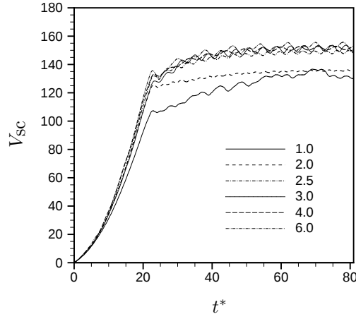
Figure 4.19: Variation of total volume of scalar carrying fluid in the domain with time. The ring velocity ratio is 0.75, duty cycle is 75% and different stroke ratios are considered.
