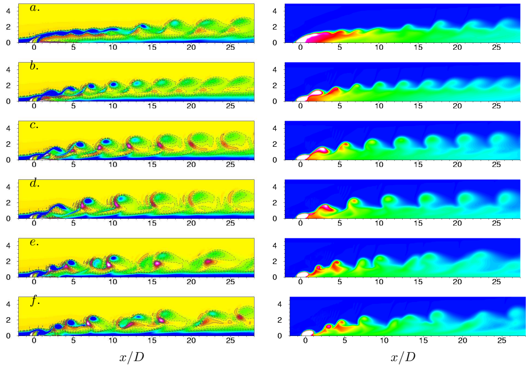
Figure 4.18: Ring velocity ratio = 0.75, duty cycle = 75%: contours of vorticity and scalar are plotted in the symmetry plane at different stroke ratios: (a) 1.0, (b) 2.0, (c) 2.5, (d) 3.0, (e) 4.0 and (f) 6.0. (The length scales on the vertical axes are all y/D .)
