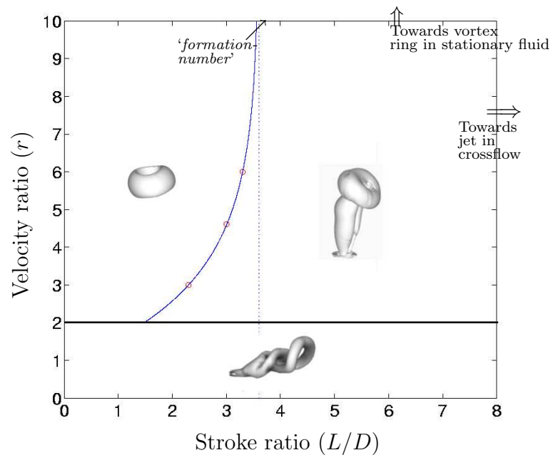
Figure 3.22: A classification map showing three regimes with different flow structure and entrainment characteristics.
