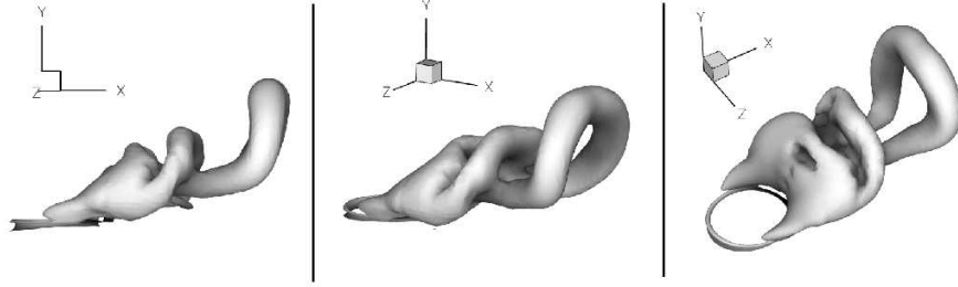
Figure 3.11: Hairpin structures are shed for L/D = 5 at r = 1 . The figures correspond to t^* = 5.0 .
