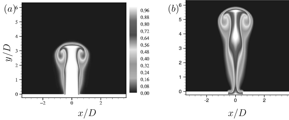
Figure 2.6: Instantaneous contours of passive scalar on z = 0 plane for L/D = 6 at t^* = (a) 6.048 and (b) 10.08. Note the trailing column behind the vortex ring.
