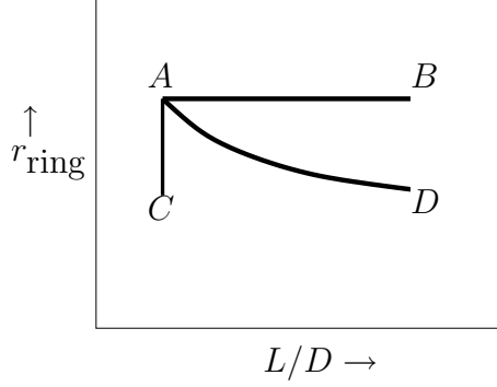
Figure 4.3: Different trajectories in ring parameter space defined in terms of stroke ratio L/D and ring velocity ratio r_{\text{ring}} .
