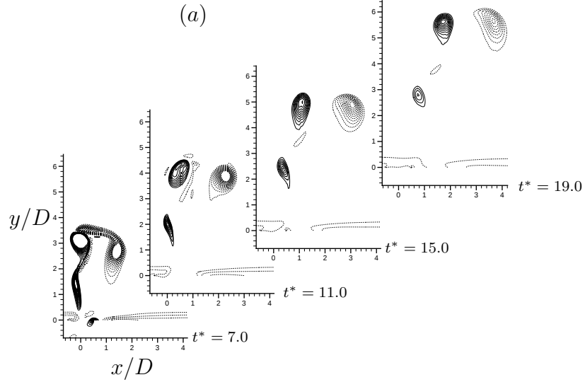
Figure 3.7: Time evolution of vorticity contours at transition stroke ratio ( L/D = 3.33 ) for r = 6 .
