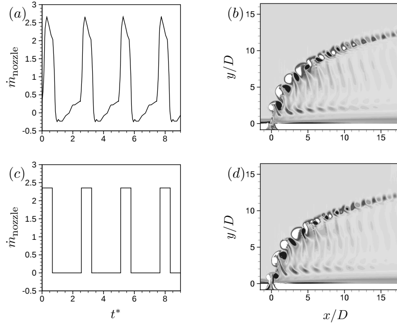
Figure 4.12: (a) & (b) Massflow rate at the nozzle exit and corresponding flow field for a waveform similar to the experiments of Shapiro et al. (2006). (c) & (d) Massflow rate at the nozzle exit and corresponding flow field for a square waveform. Both waveforms have the same stroke ratio, velocity ratio and duty cycle.
