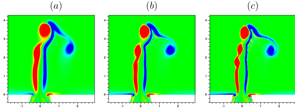
Figure 3.9: Effect of Reynolds number for L/D = 6 at r = 6 : (a) Re=600 (b) Re=900 (c) Re=1300 .
