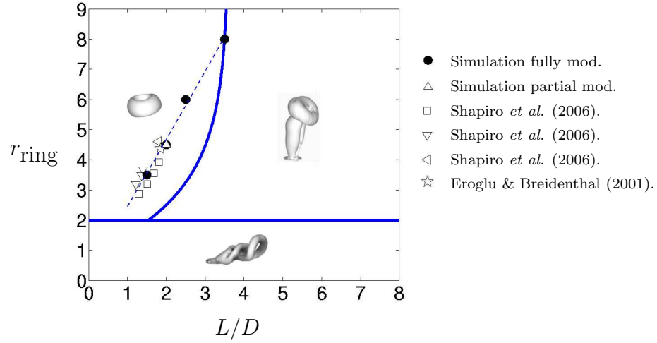
Figure 1.5: Optimal pulsing conditions from several experiments are plotted along with the optimal data from simulations. Note that the data collapse onto a curve.
