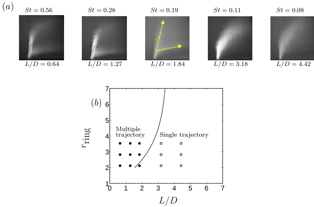
Figure 4.17: (a) Experiments of Tomar et al. (2004, reproduced by permission) on ZNMF–JIC reveal that for St \geq 0.19 (corresponds to L/D \leq 1.84 ) the mean jet structure has multiple trajectory and for St < 0.11 ( L/D > 3.18 ) the jet has single trajectory. The equivalent ring velocity ratio for this case correspond to 3.53. (b) Symbols correspond to transformed experimental data in ring parameter space. Filled and open symbols correspond to multiple and single trajectory structure respectively.
