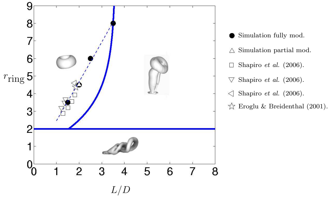
Figure 4.21: Optimal pulsing conditions from several experiments are plotted along with the optimal data from simulations. Note that the data collapse onto a curve.
