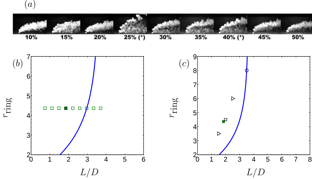
Figure 4.15: (a) Figure 6c from experiment of Shapiro et al. (2006), reprinted by permission; smoke visualization for experimental case 1, with peak-to-peak \Delta U_j fixed at 4.8 m/s with forcing frequency f = 85 Hz for duty cycle ranging from 10% to 50%. Maximum jet penetration occurs at 25% duty cycle. (b) Experimental conditions are plotted in stroke ratio and ring velocity ratio space. Filled symbol shows the optimal condition with duty cycle 25%. The solid line denotes the transition curve. (c) Optimal condition for the experiment is compared to simulations. Filled and open symbols correspond to experiment and simulations respectively.
