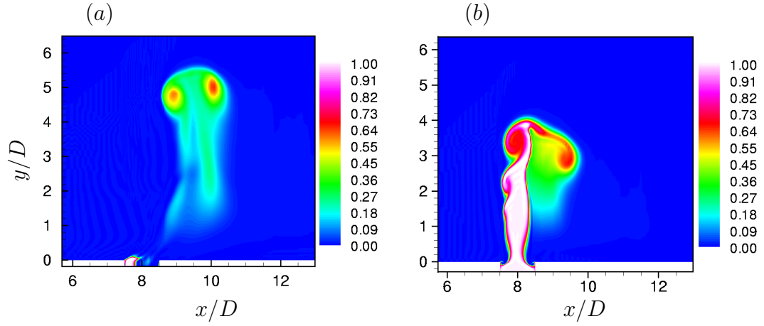
Figure 3.14: Instantaneous scalar contours on the symmetry plane for vortex ring in crossflow with r = 6 and L/D of (a) 2 & (b) 6. Note asymmetry in the scalar concentration in the case of small stroke ratio. Also note the enhanced downstream mixing for the case of large stroke ratio.
