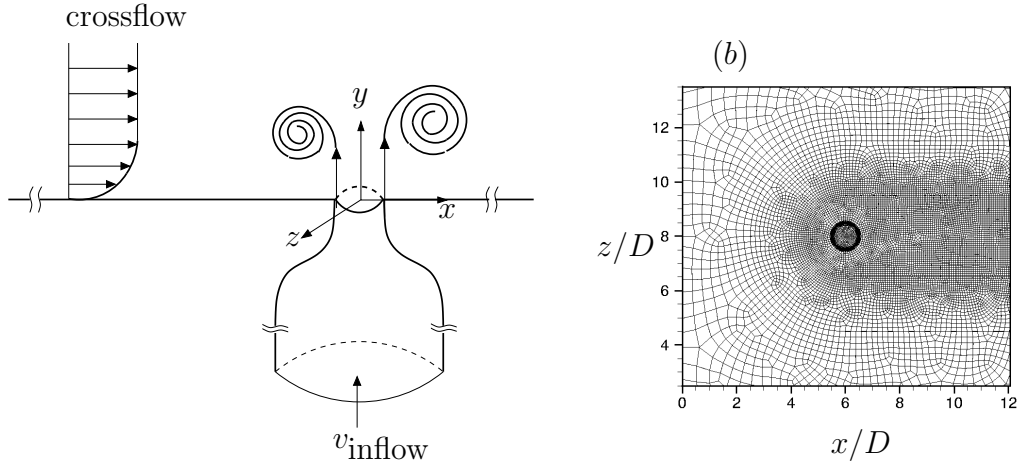
Figure 3.1: (a) Schematic of the problem. (b) Horizontal slice of the mesh.
