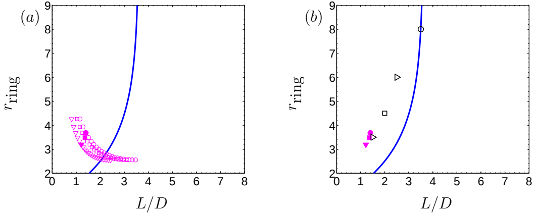
Figure 4.14: (a) Experimental conditions (case 4 of Shapiro et al. , U'_{j,\text{rms}} = 2.3 m/s) with varying pulse width for different frequencies: \circ , 87 Hz; \square , 96.7 Hz; \nabla , 124.3 Hz, are plotted in stroke ratio and ring velocity ratio space. Filled symbols show the optimal conditions with pulse width 1.6 ms. Solid line denotes the transition curve. (b) Optimal condition for the experiment is compared with simulations. Filled and open symbols correspond to experiment and simulations respectively.
