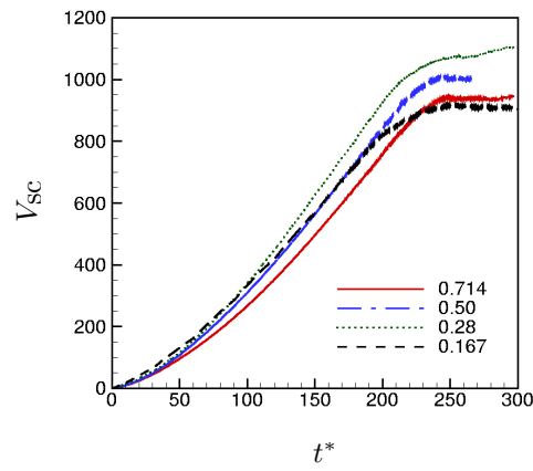
Figure 4.5: Variation of total volume of scalar carrying fluid with time. Ring velocity ratio is 8.0, duty cycle is 20% and several stroke ratios are considered.
