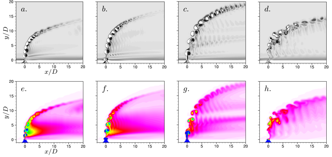
Figure 4.6: Case II: Contours of z vorticity (fig. a-d ) in symmetry plane. Ring velocity ratio, r_{\text{ring}} = 8.0 and duty cycle, \alpha = 30\% are fixed ( U_p = 3.0, U_\infty = 0.38 ). Strouhal number is varied: ( a ) & ( e ) St = 0.714 ; ( b ) & ( f ) St = 0.50 ; ( c ) & ( g ) St = 0.28 ; ( d ) & ( h ) St = 0.167 . Note that maximum penetration is achieved for St = 0.28 .
