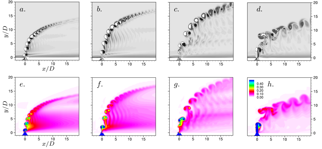
Figure 4.4: Case I: Contours of z vorticity (fig. a-d ) and scalar concentration (fig. e-h ) in symmetry plane. Ring velocity ratio, r_{\text{ring}} = 8.0 and duty cycle, \alpha = 20\% are fixed ( U_p = 3.0, U_\infty = 0.38 ). Strouhal number is varied: ( a ) & ( e ) St = 0.714 ; ( b ) & ( f ) St = 0.50 ; ( c ) & ( g ) St = 0.28 ; ( d ) & ( h ) St = 0.167 . Note that maximum penetration is achieved for St = 0.28 .
