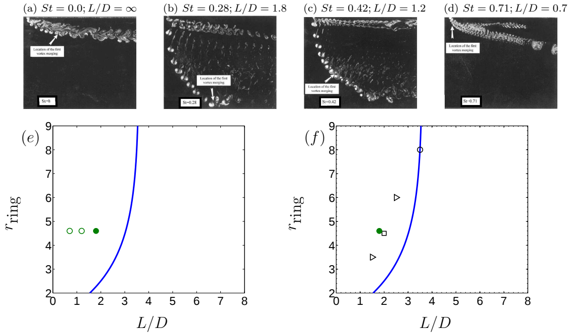
Figure 4.16: Results from the experiments of Eroglu & Breidenthal (2001, permission for reprint is being requested) showing pulsed jets in crossflow at different Strouhal numbers. Figure (a) shows the steady jet, St = 0.0 . Ring velocity ratio is 4.6 in all cases. The equivalent stroke ratios ( L/D ) are (b) 1.8, (c) 1.2 and (d) 0.7. Note figure (b) shows the maximum penetration for L/D = 1.8 .
