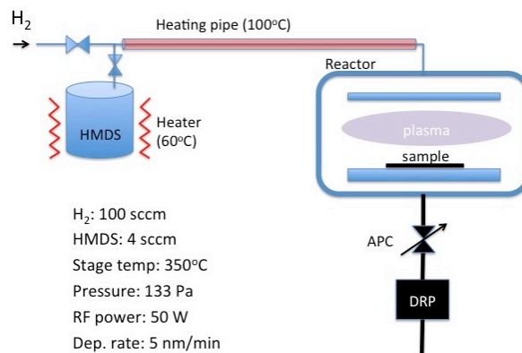
Figure 1. Diagram of PECVD system. Liquid HMDS is heated at 60°C. Vaporized HMDS is introduced into the reactor through the heated pipe. Hydrogen is also introduced into the reactor as a carrier gas. The working pressure is controlled by the automatic pressure controller (APC) and the dry vacuum pump (DRP).
