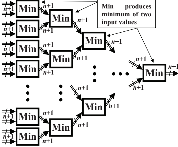
Fig. 4. Minimum circuit
