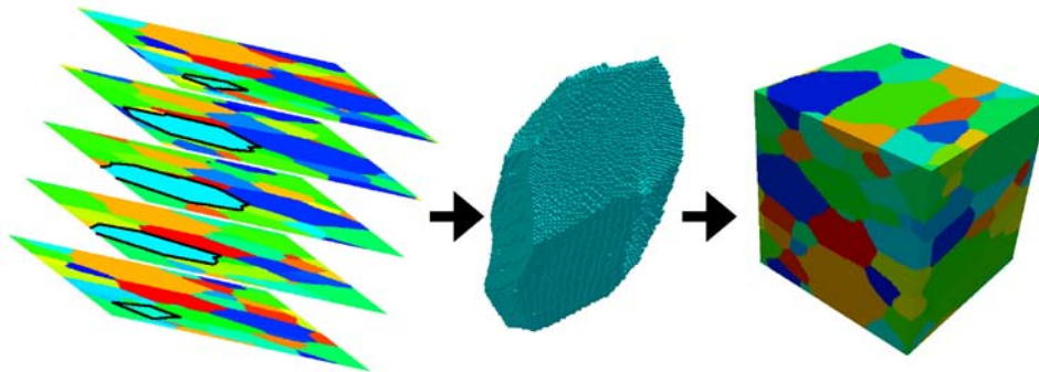
Figure 2. Schematic of the data reconstruction process for a serial sectioning experiment. A series of 2D images or data maps are collected via sequential planar material removal and characterization; only a few slices are shown that have been used to reconstruct the grain data on the right. Individual features are identified in each 2D image/map (e.g., outlined grain in data stack), and reconstructed in software to form discrete 3D data objects, which can be further grouped to reconstruct feature ensembles.
