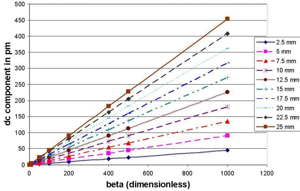
Fig 8. Variation of the static displacement component with the nonlinearity parameter for different distances of propagation for \omega = 5\text{MHz} , A_1 = 10\text{nm} .
