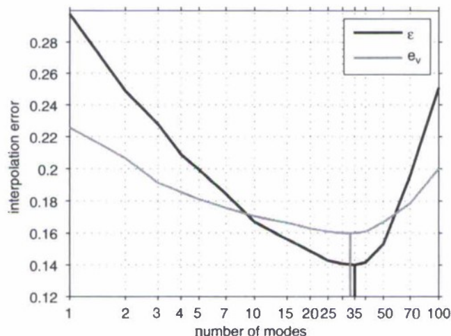
Fig. 10. Normalized interpolation errors \varepsilon and e_v as functions of the number of modes. The curves are normalized by the observed radial velocity variance \varepsilon_r .
