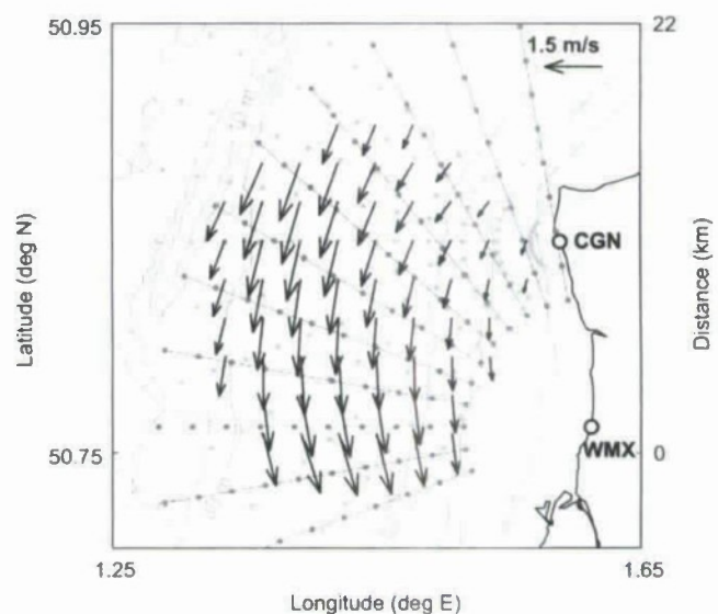
Fig. 9. Surface velocity at 12.20 GMT 24.05.2007 in the ERMANO study area. Contours show the bathymetry in meters. Gray dots indicate locations of the surface velocity measurements by two radars (shown by circles).
