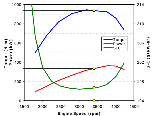
Figure 4: Prime Power Unit Torque, Speed and Fuel Consumption Map
