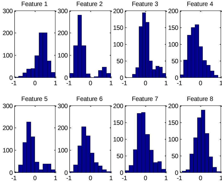
Figure 22. Feature distributions for each feature of H_1 in feature space for a non-Gaussian distributed target class.
