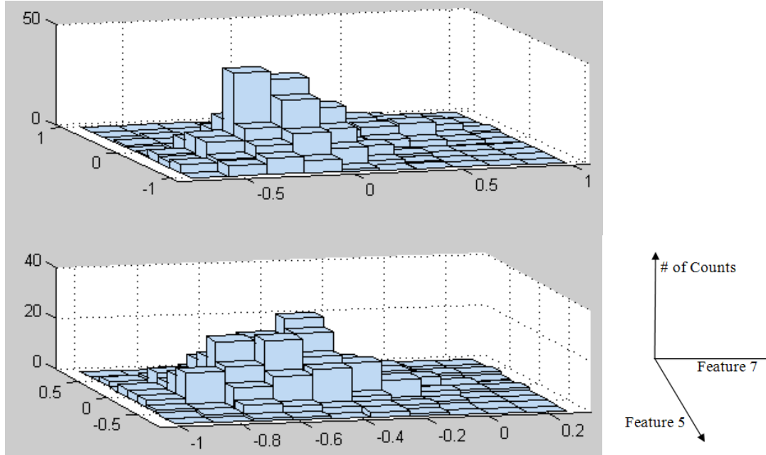
Figure 37. Two-dimensional histograms of the two classes with the selected subset of features, five and seven, obtained using the exhaustive search approach and the Bhattacharyya distance. Top and bottom histograms are for H_0 and H_1 , respectively. The diagram on the right defines the axes for the plot.
