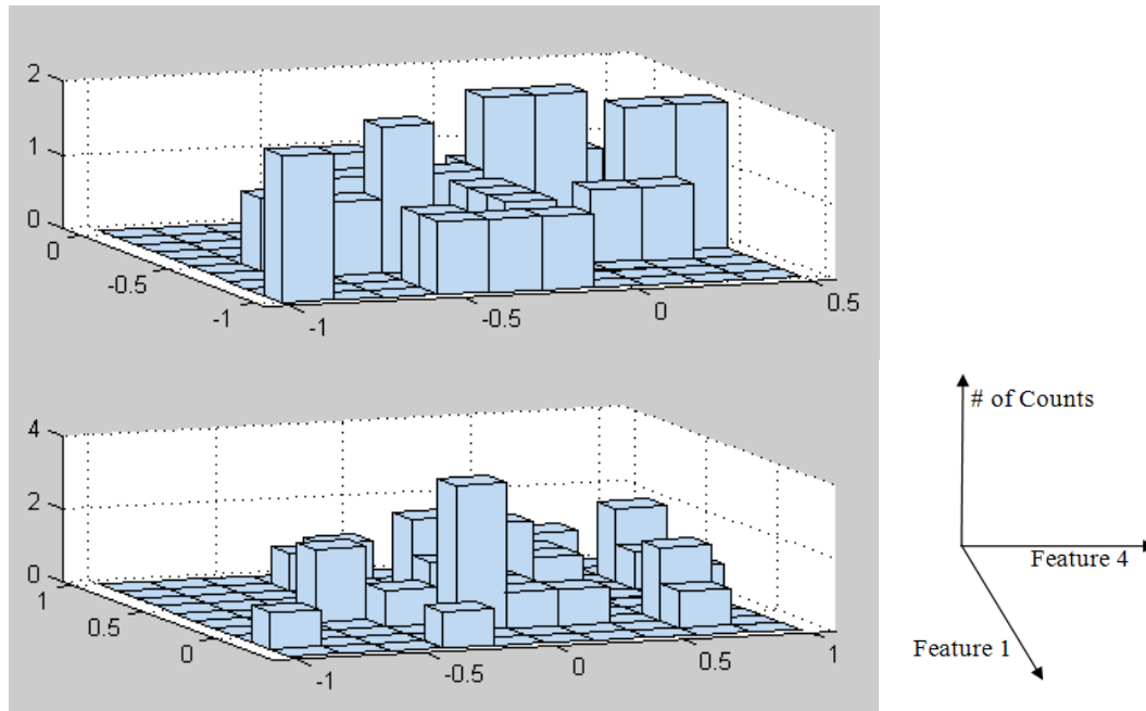
Figure 69. Two-dimensional histograms of the two classes with the selected subset of features, one and four, obtained using the exhaustive search method and the Hellinger distance. Top and bottom histograms are for H_0 and H_1 , respectively. The diagram on the right defines the axes for the plot.
