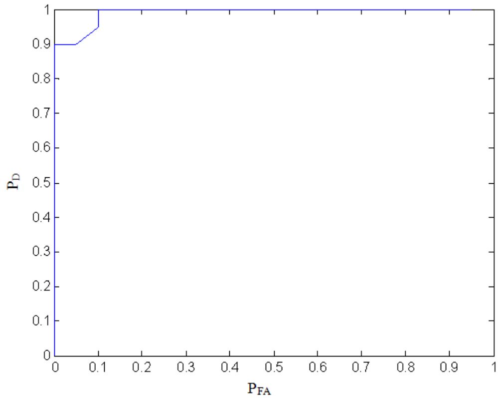
Figure 67. ROC curve for the two Fisher iris target classes using all four available features.
