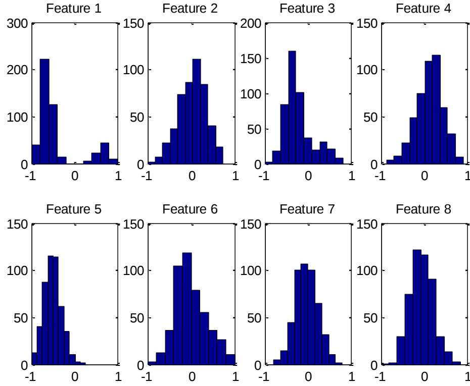
Figure 32. Feature distributions for each feature of H_1 in feature space for a non-Gaussian distributed target class.
