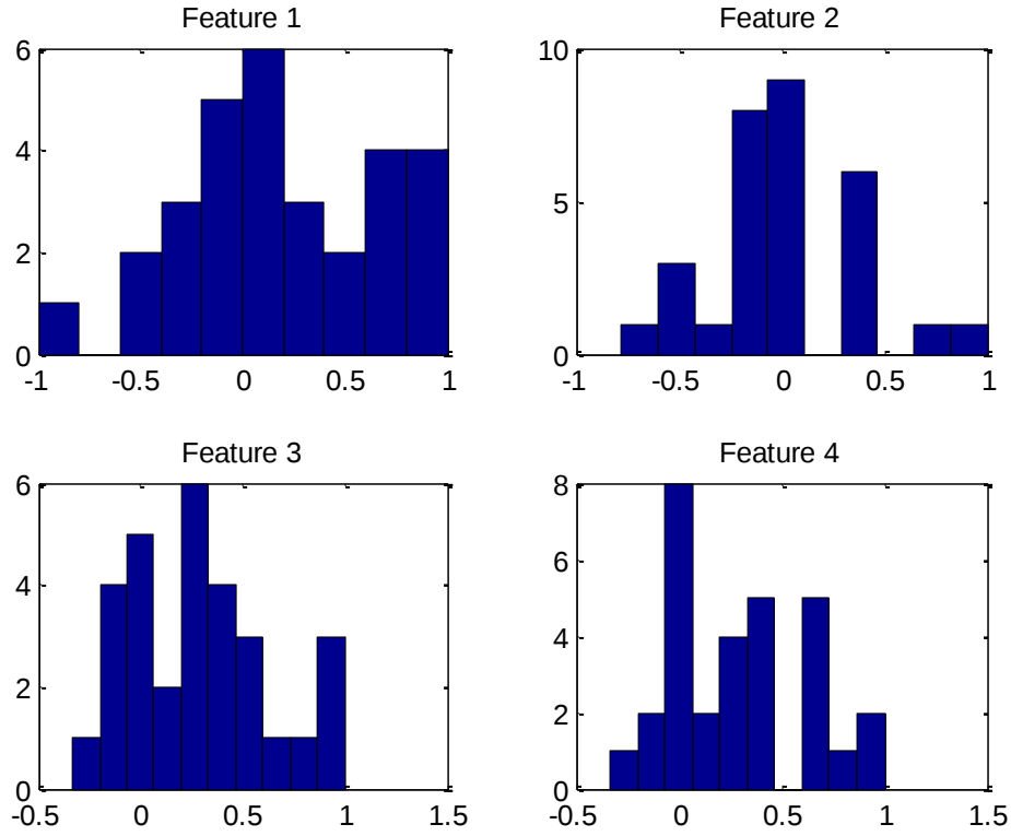
Figure 66. Feature distributions for each feature of H_1 in feature space for the Fisher iris data.
