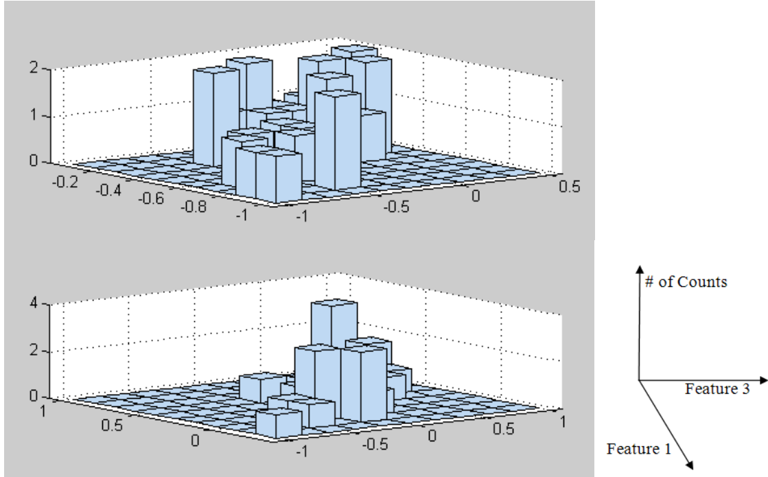
Figure 73. Two-dimensional histograms of the two classes with the selected subset of features, one and three, obtained with the exhaustive search method and the Bhattacharyya distance. Top and bottom histograms are for H_0 and H_1 , respectively. The diagram on the right defines the axes for the plot.
