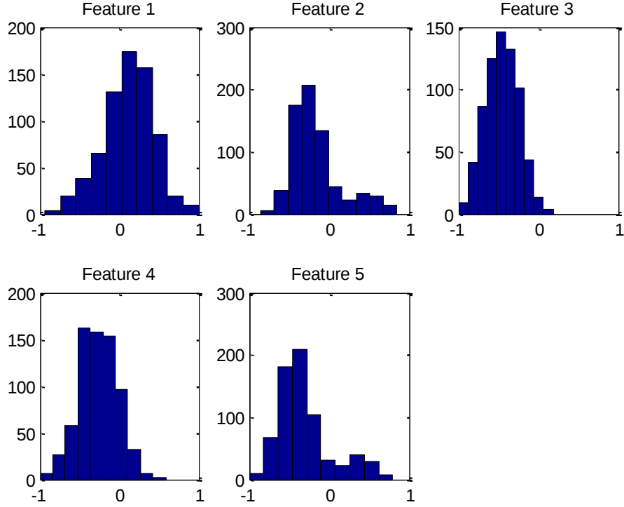
Figure 54. Feature distributions for each feature of H_1 in feature space for a non-Gaussian distributed target class.
