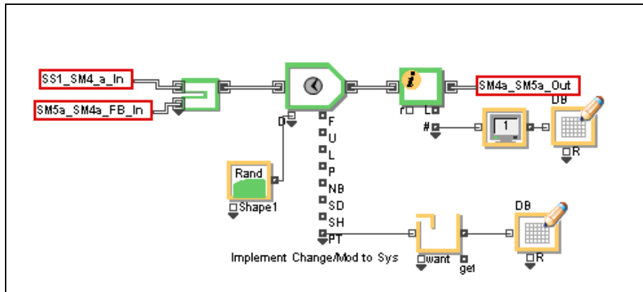
Figure 35: ExtendSim Model for Sys4: Implement Changes/Modifications to System (Level 2)
