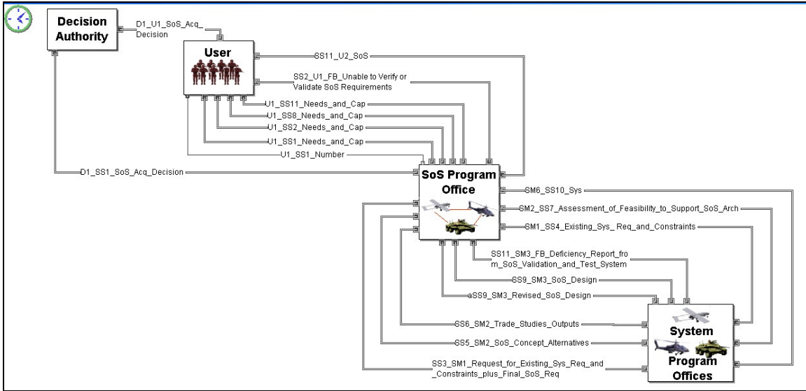
Figure 18: ExtendSim Model for Proposed SoS SE Process (Level 0 – Overview)
