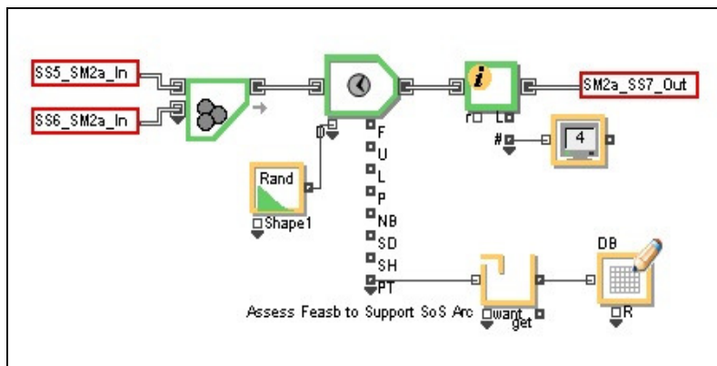
Figure 53: ExtendSim Model for Sys2: Assess Feasibility to Support SoS Architectures (Level 2)
