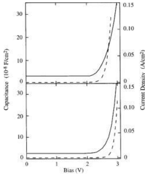
Figure 9. Capacitance-Voltage and Current-Voltage Characteristics [From 10].
