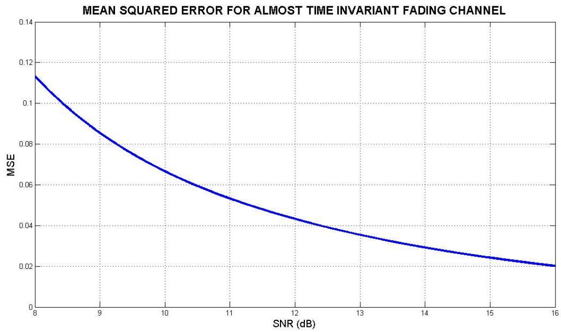
Figure 39. MSE for dual input Kalman estimator with time invariance
