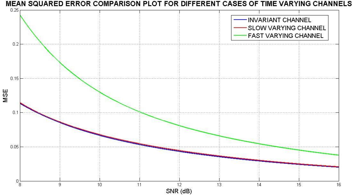
Figure 45. Comparison plot of MSEs for different time-varying channels
