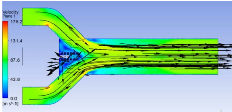
Figure 16. Fluid Flow With Velocity for Four-Inlet Arm System
