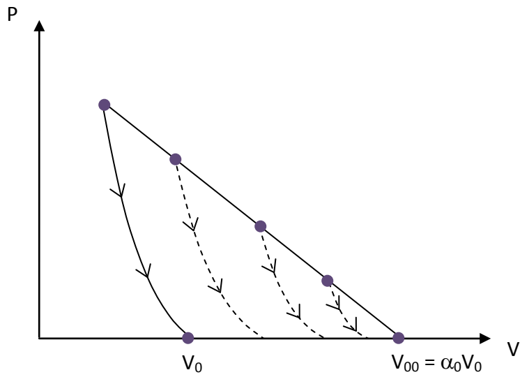
Figure 25. Possible variations in release paths for porous materials
