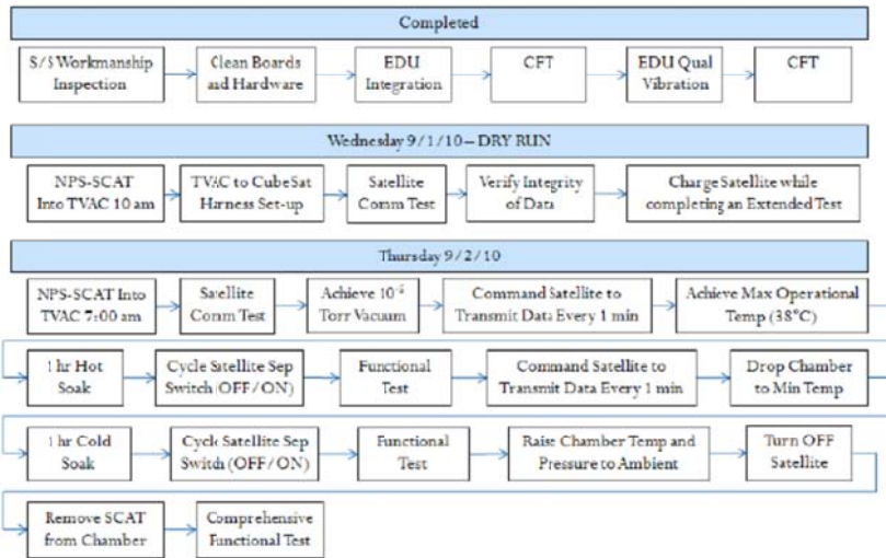
Figure 1: EDU TVAC Testing Task Flow
