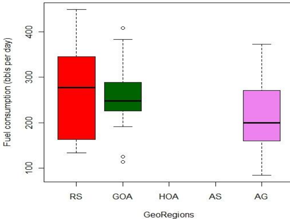
Figure 26. Side by side box plots signifying DFM fuel consumption. The chart implies no discernable differences within sub-regions.
