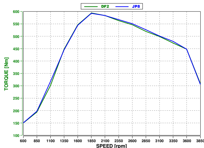
Figure 1: Modified 3.0L Torque Curve.
