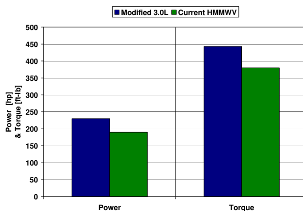
Figure 2: Gross Power and Torque Comparison vs. Current HMMWV Configuration
