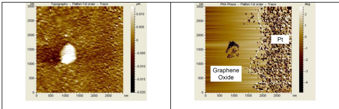
Figure 3. Micrograph of surface morphology by AFM (Left), and impedance (Right) measured at f=2.375538 GHz. Due to the thin thickness of graphene oxide ( \sim 1\text{nm} ), the boundary between graphene oxide and Pt is hardly seen by AFM. Applying RF/microwave signals, the boundary is clearly revealed on the impedance measurements because of the difference of the electrical conductivity between the graphene oxide and platinum.
