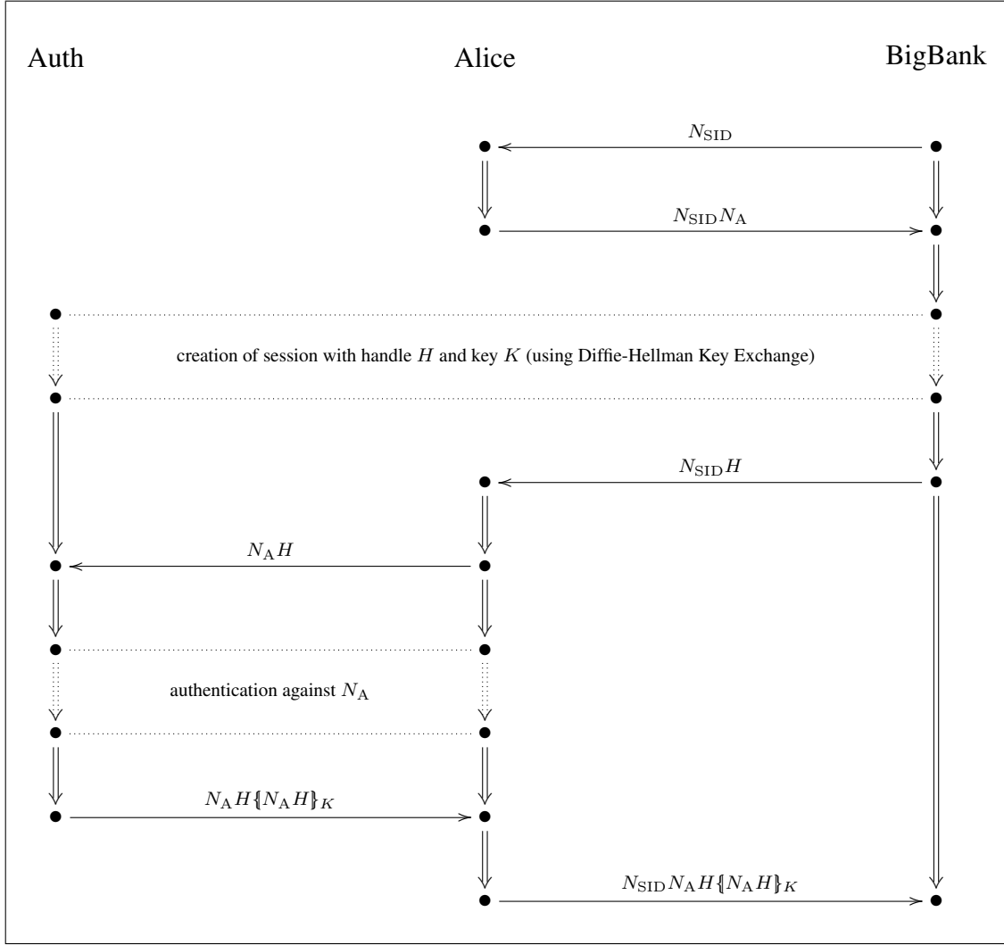
Figure 4.4: Using OpenID for Authentication
