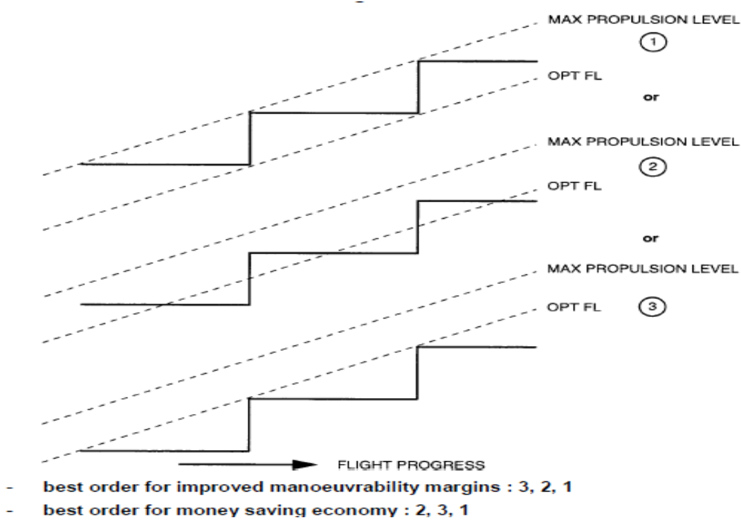
Figure 5. Step-Climb Profiles (3, 27)
