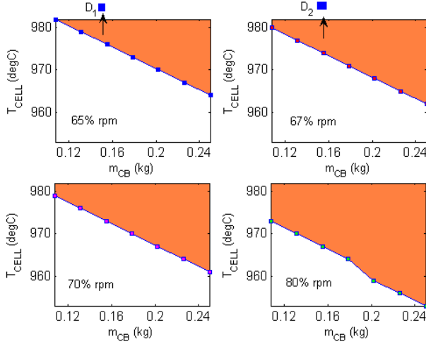
Fig. 7. ROA lower boundary for a dual-shaft SOFC/GT model for P_{NET}=5.7\text{kW} and (W_{Fuel}, I_{COM}, P_{GEN})=(0.0021, 2000, 50) . The equilibrium point is (rpm, T_{CELL} , m_{CB} )=(67% rpm, 1042degC, 0.15kg).
