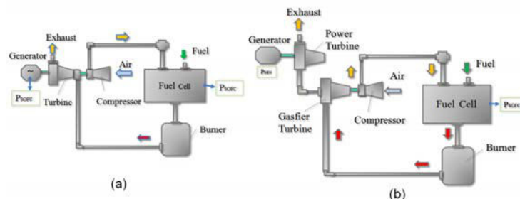
Fig. 1. SOFC/GT Hybrid schematic: single-shaft (a) and dual-shaft (b).
