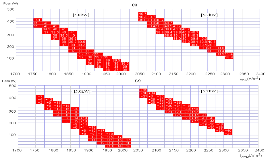
Fig. 4. The single-shaft operating regime to produce the net powers of 5.0kW and 5.7kW. (a) system efficiency map, (b) fuel cell temperature variation ( T_{CELL} -1000degC) as functions of SOFC current density and a generator load.
