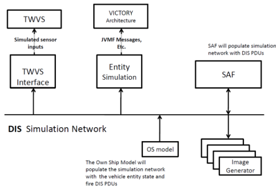
Figure 4: ISSIL Testing Using Dynamic SAF Environment
