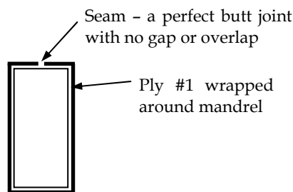
Figure 15: Diagram of the cross-section of a well wrapped mandrel
