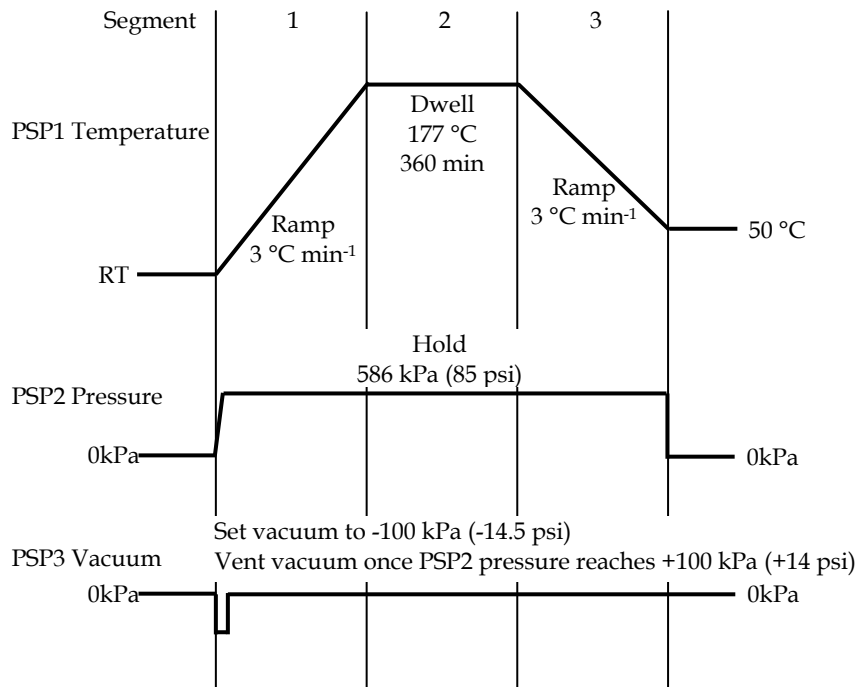
Figure 21: Autoclave cure cycle for Cycom IM7/977-3
