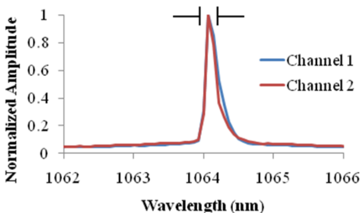
Fig. 9. (left) Emission spectra (limited by the spectrometer resolution) and (right) fringe pattern of the two channels for coherent locking using 2 nd order M-VBG.
