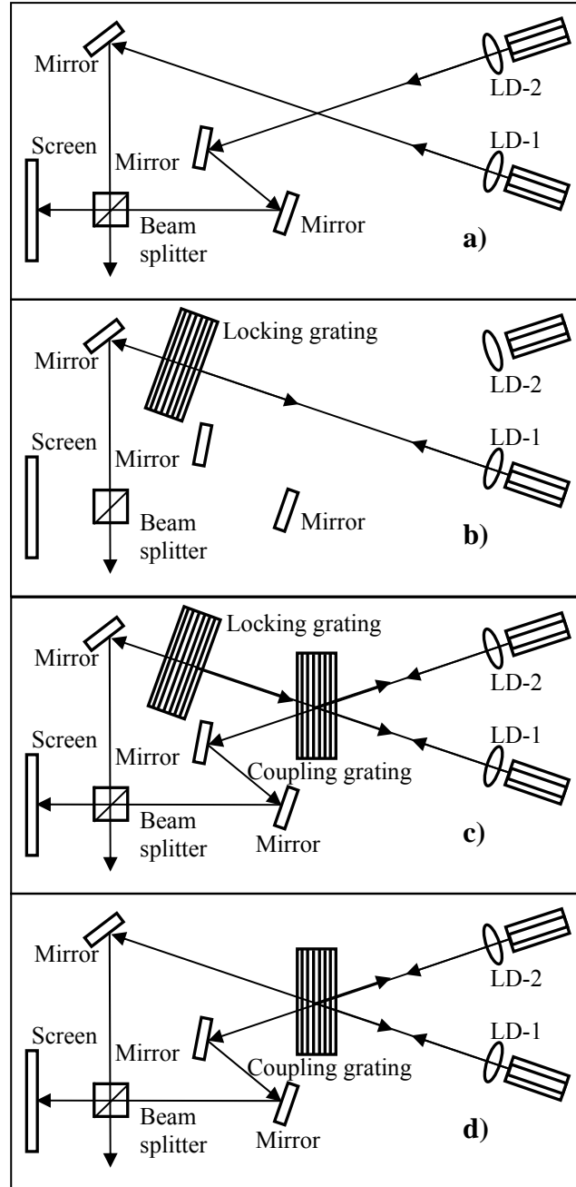
Fig. 2. Optical scheme of coherent coupling of laser diodes: a) – combining of independent diodes, b) – spectral locking of LD-1, c) – spectral locking of LD-1 and phase locking of two diodes, d) phase locking of two diodes.
