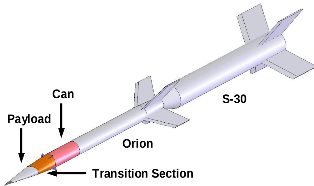
Figure 3 HIFiRE-5 stack.
