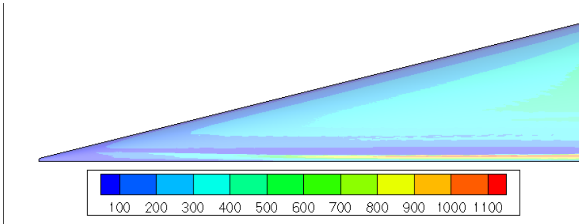
Figure 58 Crossflow Reynolds number contours for 33 km case
