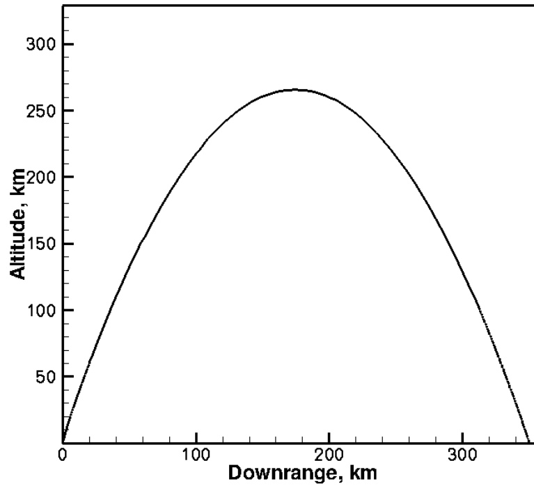
Figure 8 HIFiRE 5 trajectory
