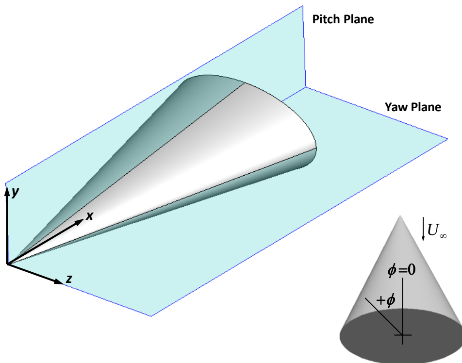
Figure 4 Elliptic cone geometry and coordinate system.
