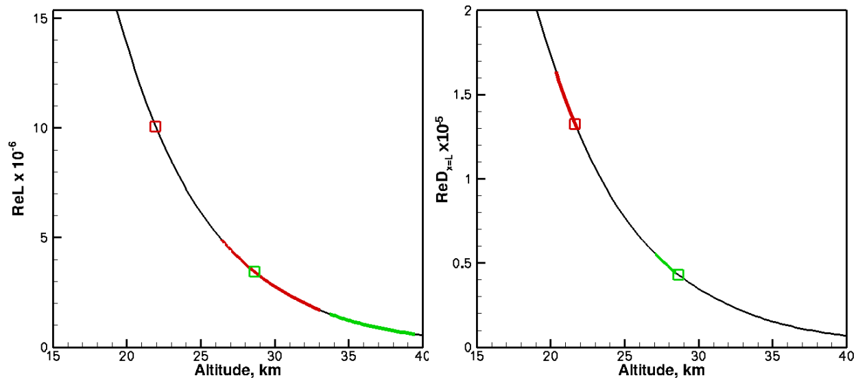
Figure 30 Length Reynolds number (left) and leading edge diameter Reynolds number (right) as functions of altitude.
