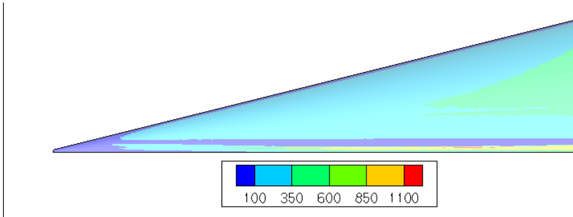
Figure 57 Crossflow Reynolds number contours for 28km case
