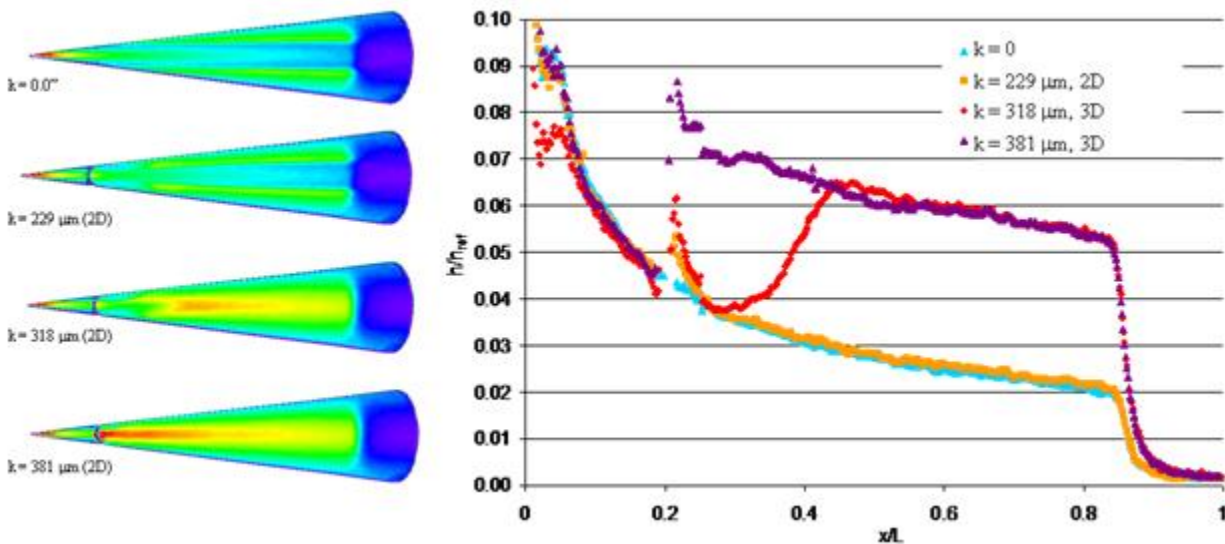
Figure 27: Boundary Layer Trip Effectiveness for the Side Surface, 4 deg Beta, \text{Re} = 18.4 \times 10^6/\text{m}
