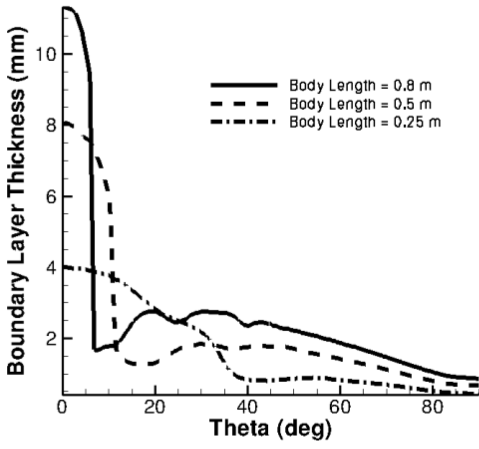
Figure 40 Boundary layer thickness at select locations along the length of the body for 33km case. Theta the radial coordinate from 0 (centerline) to 90 (leading edge).
