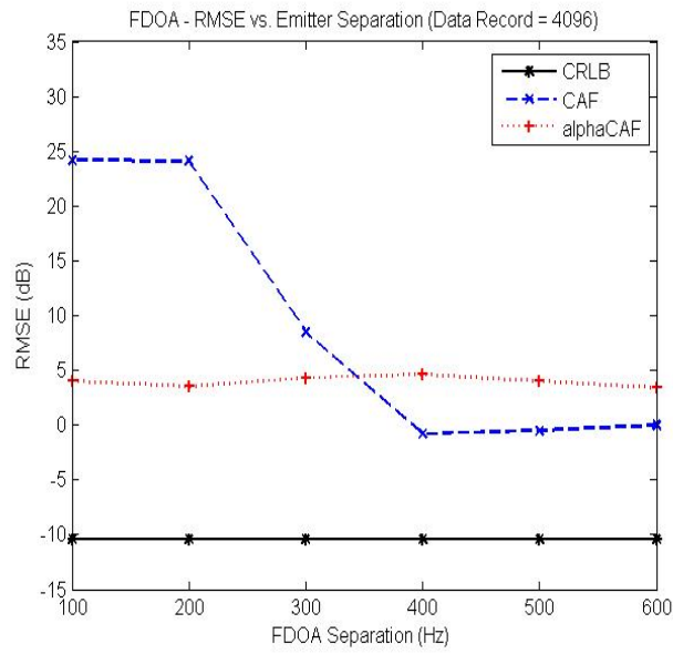
Figure 6.14: FDOA estimate RMSE versus FDOA separation for SOI and SNOI scenario computed using 1000 trials for each record length and an SIR = 0 dB at both receivers.
