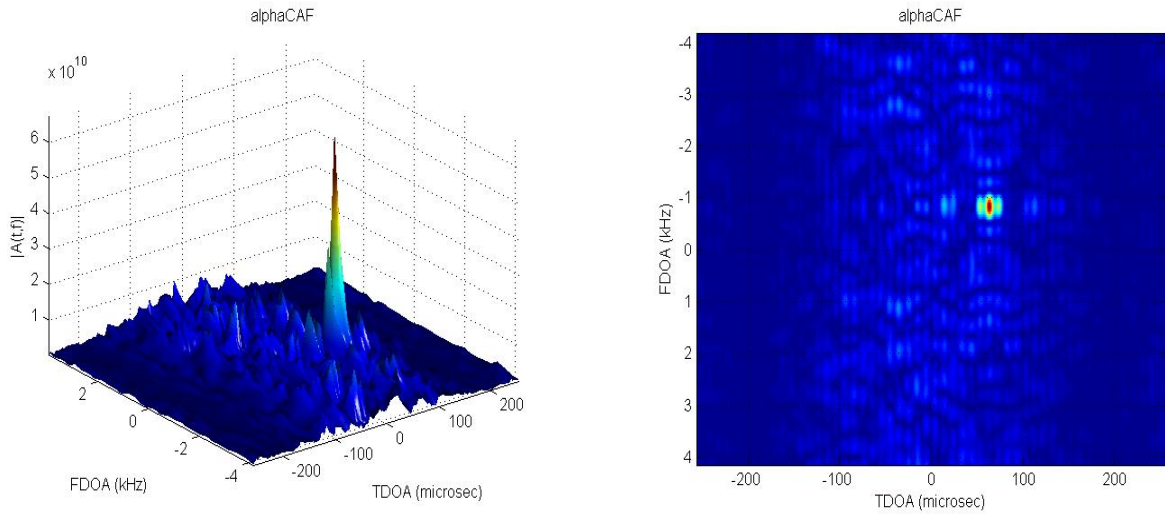
Figure 4.3: alphaCAF surface computed from SNOI only with \text{SNR} = 5 dB. Cyclic frequency was fixed at the SOI symbol rate ( 26/256f_s ). The data record length is 2048 samples with a sample rate of 1 MHz (Left). Top view of surface to the left (Right).
