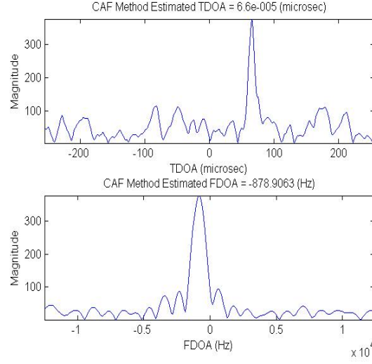
Figure 2.19: Cross-section plots through the Figure 2.18 CAF surface in both the TDOA and FDOA dimensions.
