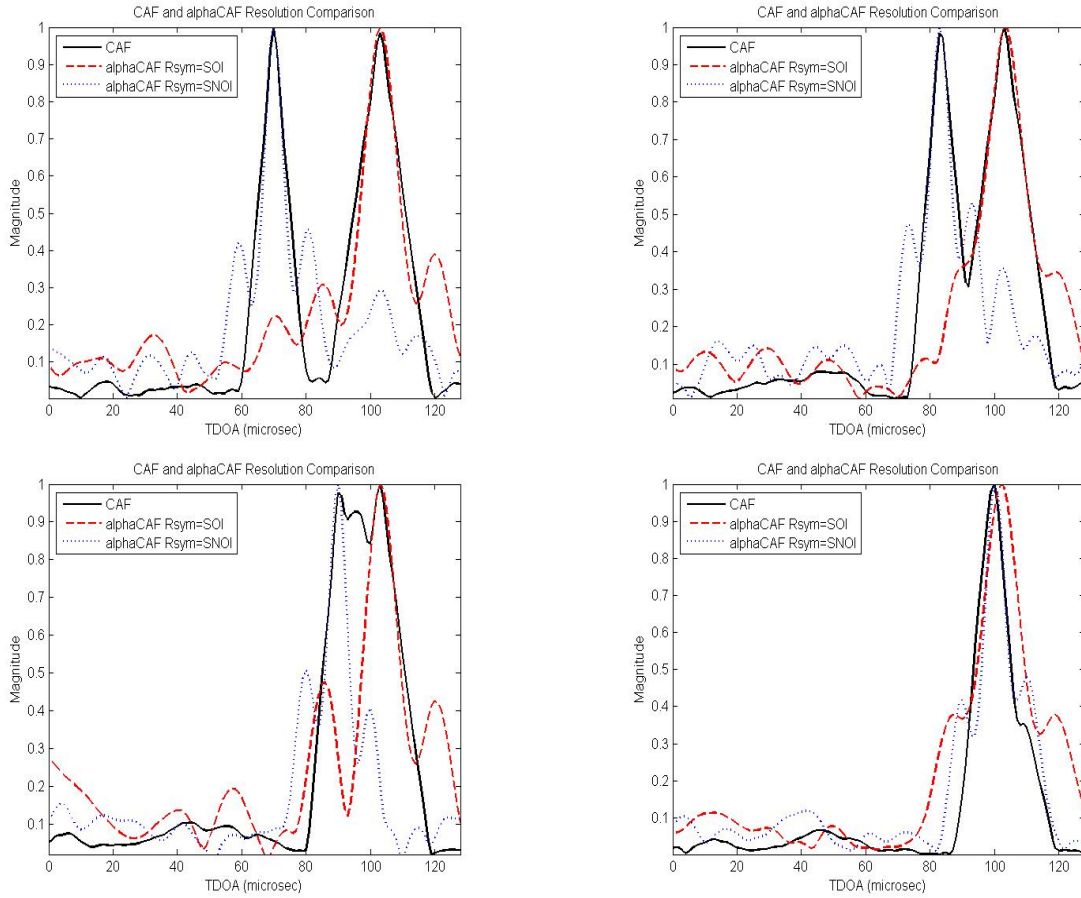
Figure 6.3: Demonstration of alphaCAF resolution performance compared to conventional CAF using data record length of 2048 samples at 1MHz sample rate. The TDOA difference between the SOI and SNOI goes from large to small starting at the top left plot, getting smaller from left to right.
