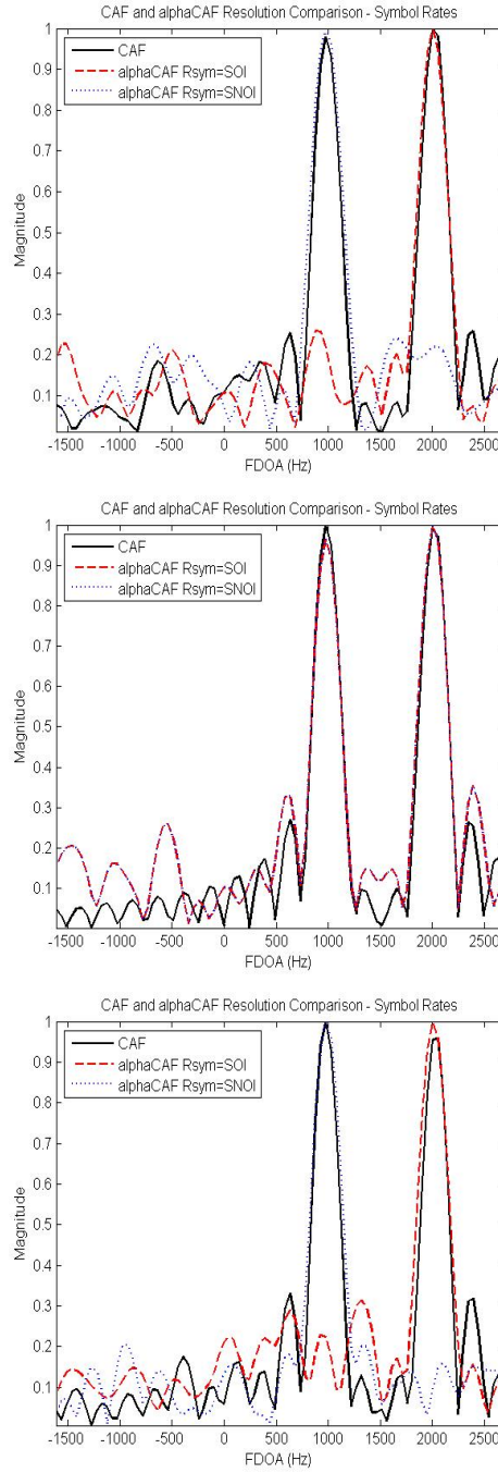
Figure 6.6: Demonstration of alphaCAF resolution performance compared to conventional CAF using data record length of 4096 samples at 1 MHz sample rate. The FDOA difference between the SOI and SNOI is fixed to be large enough that the CAF method can easily generate separate peaks. The SOI symbol rate is fixed at 16/256 the sample rate. The SNOI symbol rate is shown for 15.2/256 f_s , 16/256 f_s , 16.8/256 f_s from top to bottom respectively.
