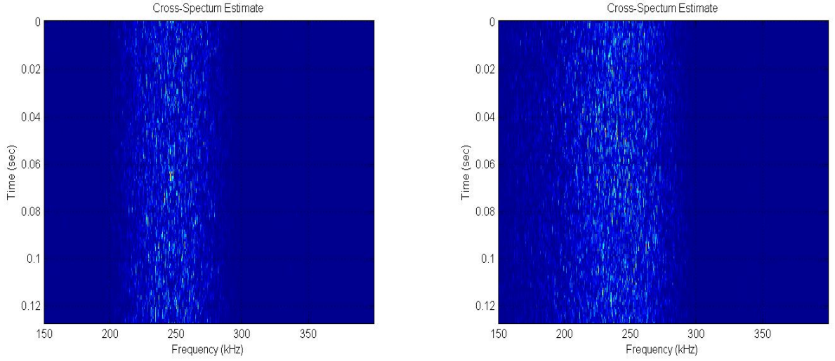
Figure 2.22: Cross spectrum magnitude vs.time representation for SOI used in hybrid method examples (Left). Cross spectrum vs.time representation for combined SOI and SNOI used in this section's hybrid method examples (Right).
