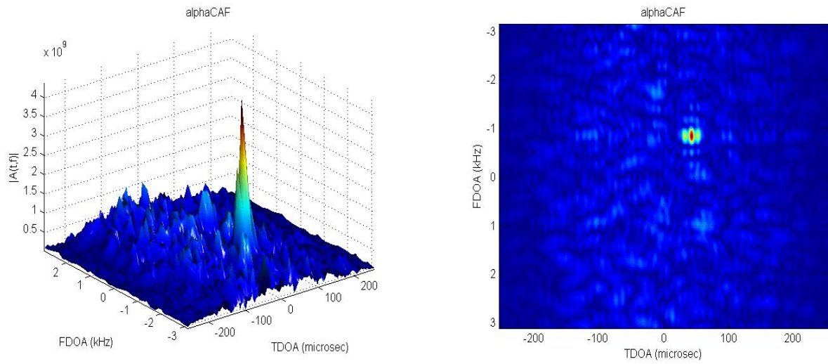
Figure 4.11: alphaCAF output computed for spatially separated SOI and SNOI. The \text{SIR} = 0 dB for both receivers. The cyclic frequency was fixed at the SNOI symbol rate in order to separate the SOI estimate. The data record length is 2048 samples with a sample rate of 1 MHz (Left). Top view of surface on the left (Right).
