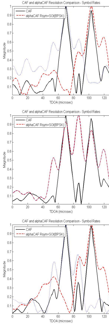
Figure 6.5: Demonstration of alphaCAF resolution performance compared to conventional CAF using data record length of 4096 samples at 1 MHz sample rate. The TDOA difference between the SOI and SNOI is fixed to be large enough that the CAF method can easily generate separate peaks. The SOI symbol rate is fixed at 16/256 the sample rate. The SNOI symbol rate is shown for 15.2/256fs , 16/256fs , 16.8/256fs from top to bottom respectively.
