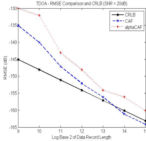
Figure 6.9: SOI only TDOA estimate RMSE versus data record length computed using 1000 trials for each record length and an SNR = 20 dB at both receivers.
