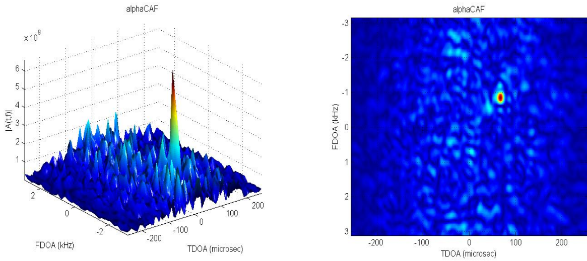
Figure 4.5: alphaCAF surface computed from SOI and SNOI with the cyclic frequency fixed at the SOI symbol rate in order to separate the SOI estimate. The SIR = 0 dB for both receivers. The data record length was 2048 samples with a sample rate of 1 MHz (Left). Top view of surface to the left (Right).
