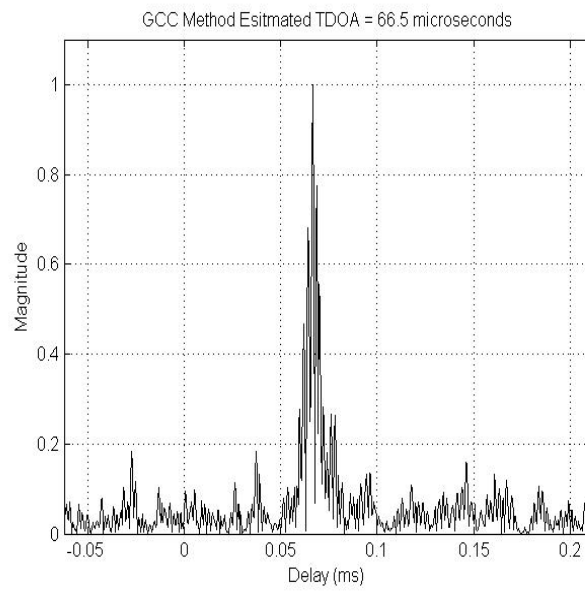
Figure 2.7: GCC SCOT output for the BPSK SOI and BPSK SNOI listed in Table 2.2 and collected by two spatially separated stationary receivers. The data record length was 2048 samples and the \text{SNR} = 20 dB at both receivers. Both receiver sample rate were 1 MHz. The distance between the SOI and SNOI emitters is 0.5 km.
