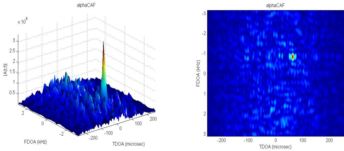
Figure 4.7: alphaCAF surface computed from SOI and SNOI with the cyclic frequency fixed at the SNOI symbol rate in order to separate the SNOI estimate. The SIR = 0 dB for both receivers. The data record length was 2048 samples with a sample rate of 1 MHz (Left). Top view of surface to the left (Right).
