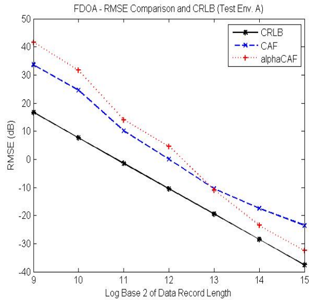
Figure 6.12: SOI FDOA estimate RMSE versus data record length computed using 1000 trials for each record length and for test environment A. SIR = 0 dB at both receivers.
