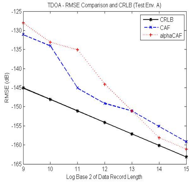
Figure 6.11: SOI TDOA estimate RMSE versus data record length computed using 1000 trials for each record length and for test environment A. SIR = 0 dB at both receivers.
