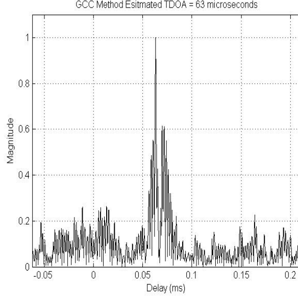
Figure 2.6: GCC SCOT output for the BPSK SOI and BPSK SNOI listed in Table 2.2 and collected by two spatially separated stationary receivers. The data record length was 2048 samples and the \text{SNR} = 20 dB at both receivers. Both receiver sample rate were 1 MHz. The distance between the SOI and SNOI emitters is 1 km.
