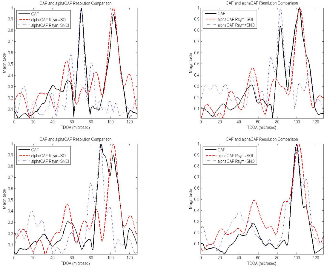
Figure 6.1: Demonstration of alphaCAF resolution performance compared to the conventional CAF using a data record length of 2048 samples at a sample rate of 1MHz. The TDOA difference between the SOI and SNOI varies from large to small starting at the top left plot, getting smaller from left to right.
