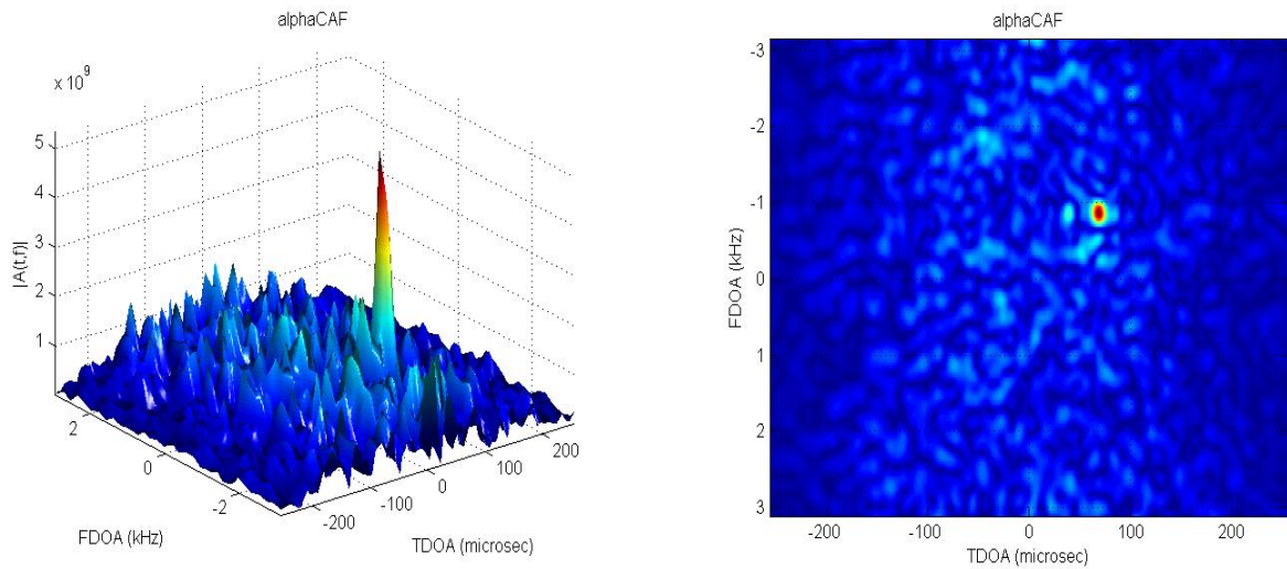
Figure 4.10: alphaCAF output computed for spatially separated SOI and SNOI. The SIR = 0 dB for both receivers. The cyclic frequency was fixed at the SOI symbol rate in order to separate the SOI estimate. The data record length is 2048 samples with a sample rate of 1 MHz (Left). Top view of surface on the left (Right).
