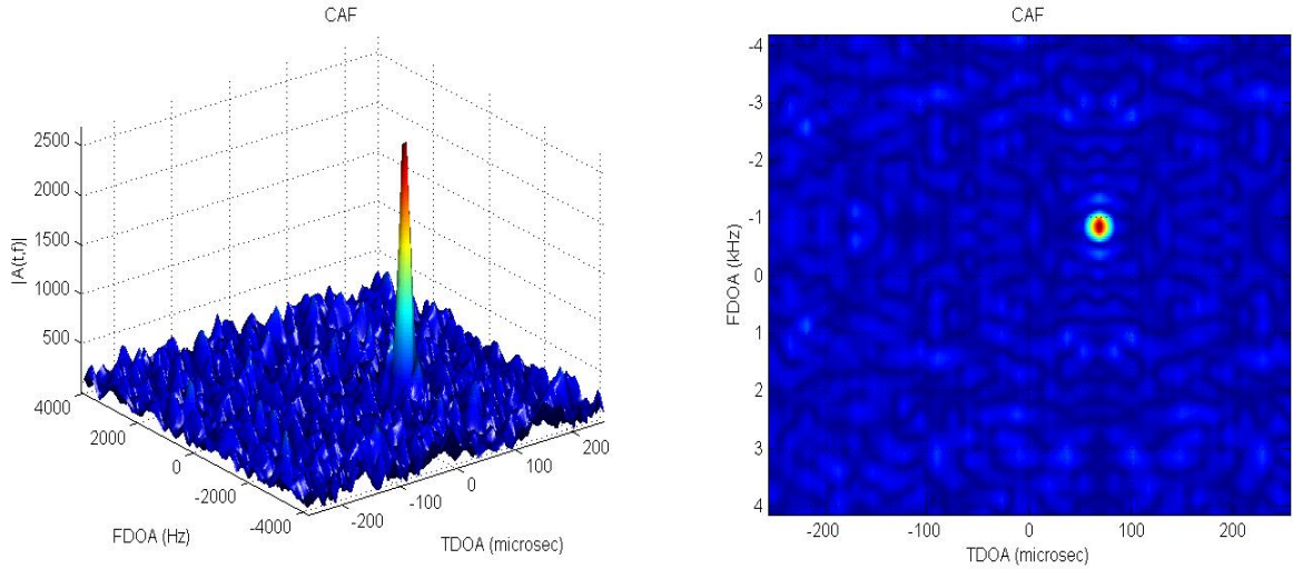
Figure 2.10: CAF surface for BPSK SOI collected at two spatially separated receivers with an \text{SNR} = 20 dB at both receivers. The data record length was 2048 samples and the receiver sample rates were 1 MHz. The peak location in the surface corresponds to the TDOA and FDOA estimates. (Left). Top view of CAF surface on the left (Right).
