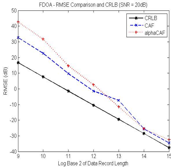
Figure 6.10: SOI only FDOA estimate RMSE versus data record length computed using 1000 trials for each record length and an SNR = 20 dB at both receivers.
