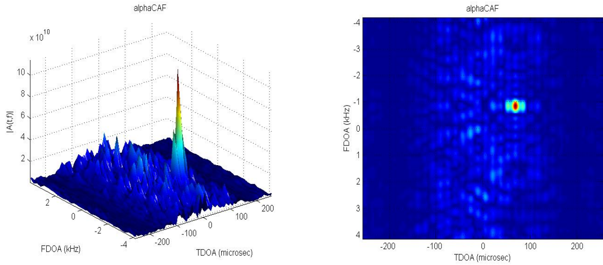
Figure 4.1: alphaCAF surface computed from SOI only with SNR = 5 dB. Cyclic frequency was fixed at the SOI symbol rate ( 16/256f_s ). The data record length is 2048 samples with a sample rate of 1 MHz (Left). Top view of surface to the left showing peak location corresponding to TDOA and FDOA estimate (Right).
