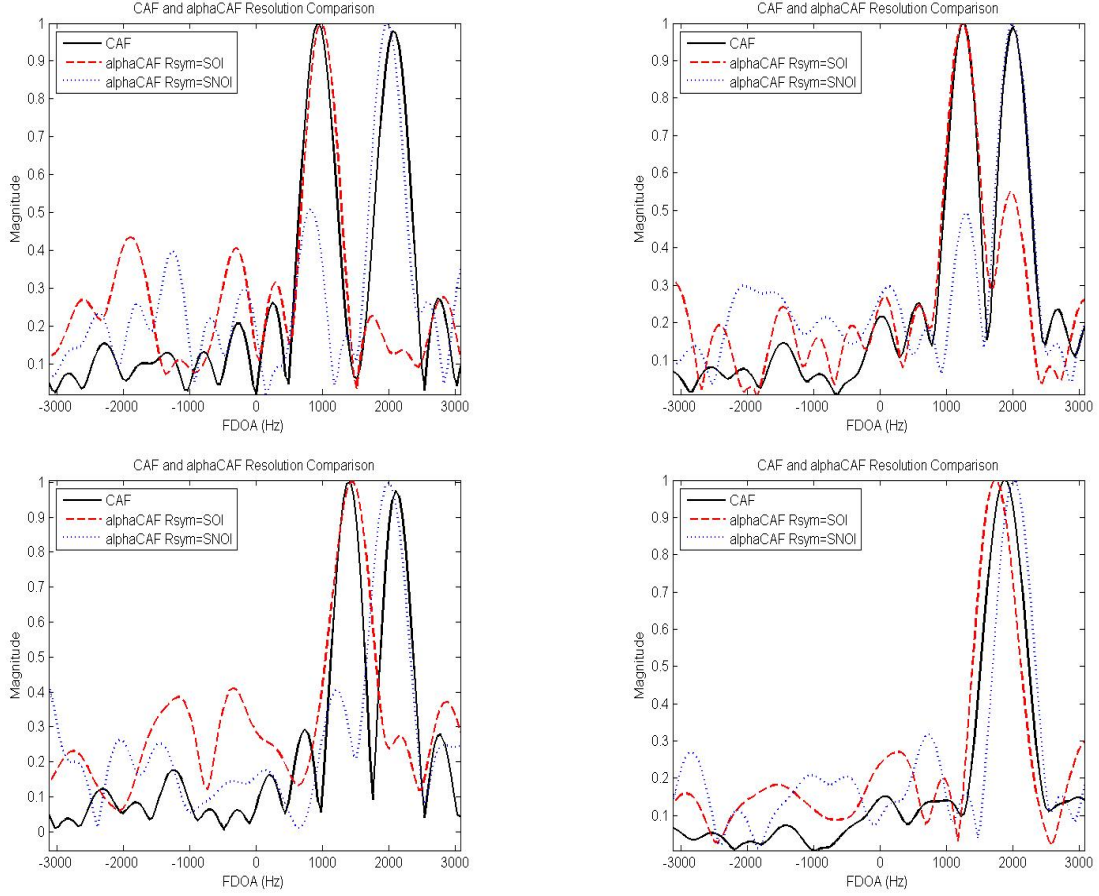
Figure 6.2: Demonstration of alphaCAF resolution performance compared to the conventional CAF using a data record length of 2048 samples at a sample rate of 1 MHz. The FDOA difference between the SOI and SNOI varies from 1000 Hz to 250 Hz starting at the top left plot, getting smaller from left to right.
