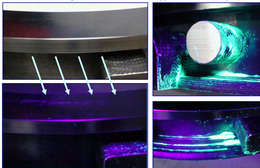
Figure 36: EBWD Prototype Case FPI Inspection Evaluation
