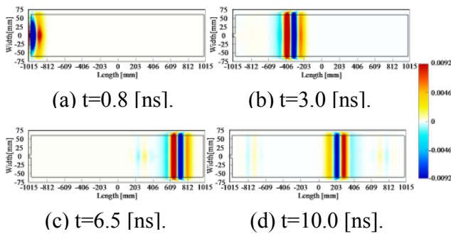
Fig. 10 Analysis E_z of z=0 plane ( l=18 [mm]).
