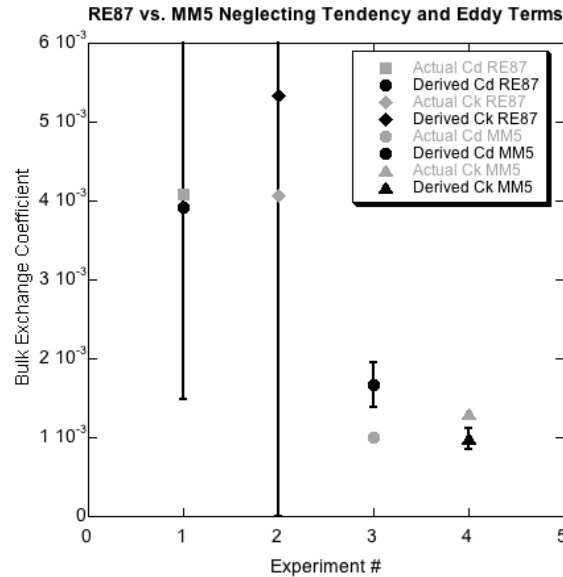
Figure 3: Estimated (gray) and derived (black) surface exchange coefficients, with error estimates. From left to right: drag coefficient and enthalpy exchange coefficient from the axisymmetric model, drag coefficient and enthalpy exchange coefficient from a simulation using the MM5 model.
