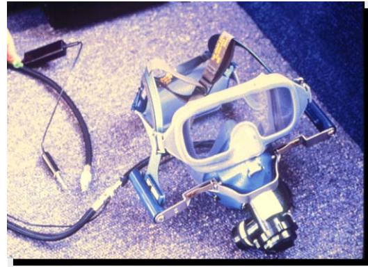
Figure 5.2.6-1. 358 Series Quick-Don Figure 5.2.6-2. 359 Series Quick-Don
