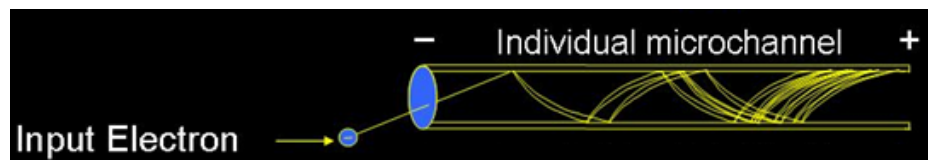
Figure 6.1.1-2. Microchannels
