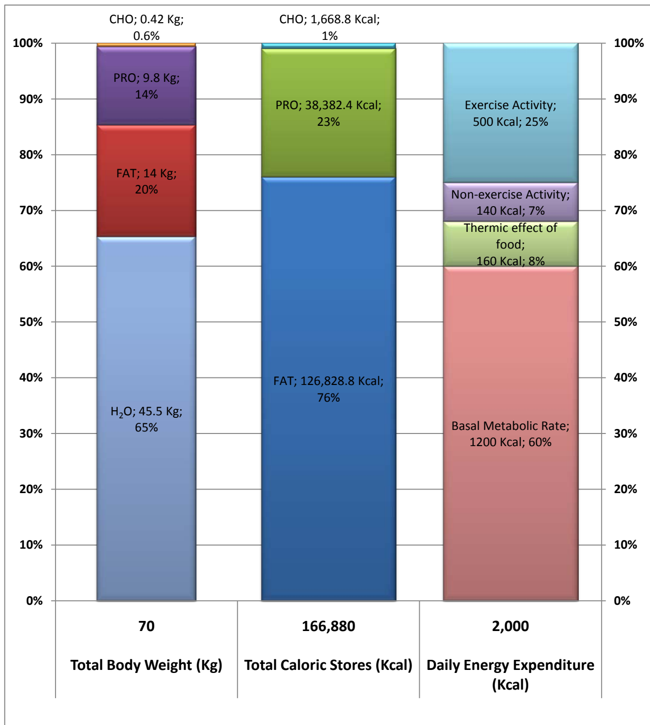
Figure 1.6.17-2. Composition of an Average 70-kg Individual
