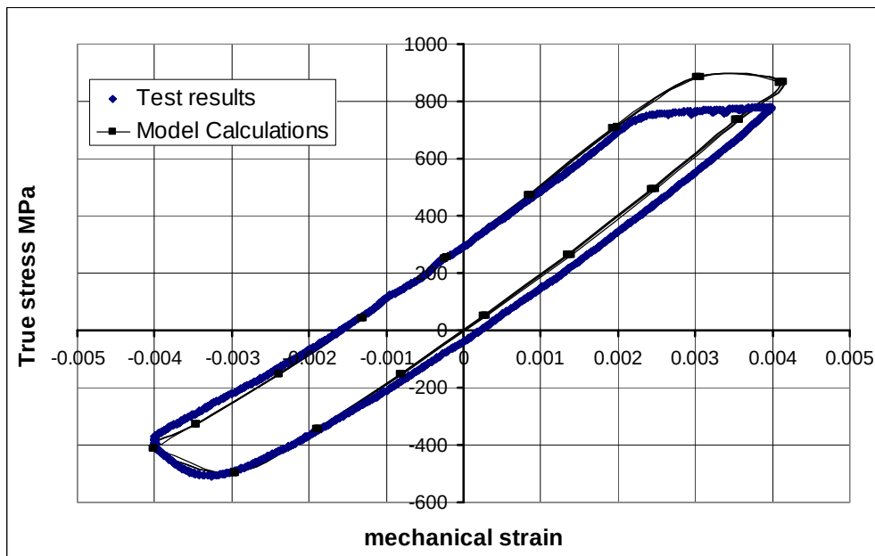
Figure 16. Predicted stress-strain curve against test data for OP TMF test up to 0.4% mechanical strain range along (\bar{1}23) crystallographic direction at the temperature range from 427 C to 1038 C
