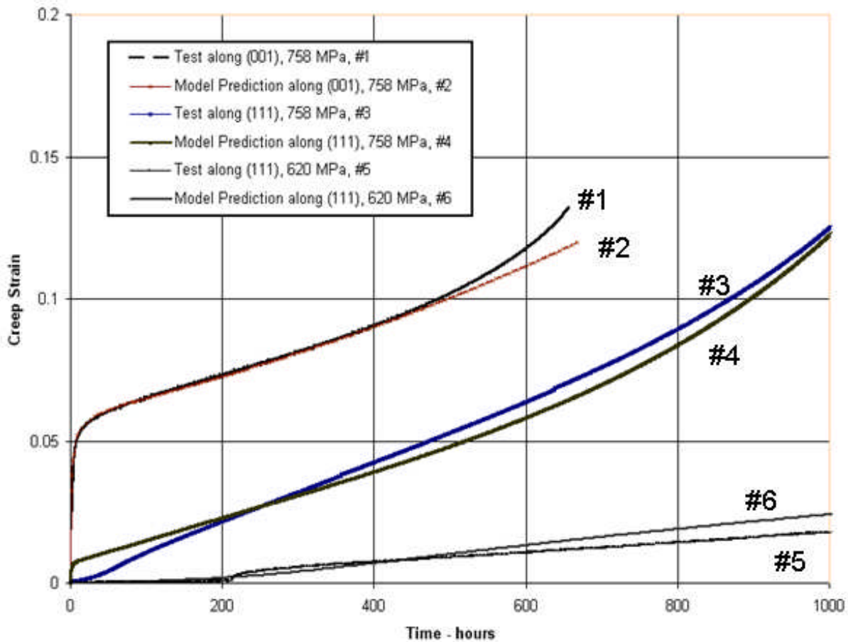
Figure 3. Model predictions and creep test results at temperature 760 C. Lines #1 and #2 are tests and simulation results correspondingly of creep along (001) crystallographic direction with nominal (initial) stress of 758 MPa. Lines #3 and # 5 are creep test results along (111) direction conducted at nominal stress levels of 758 MPa and 620 MPa correspondingly. Lines #4 is the simulation results for the test #3 and line #6 is the results of simulations for the test curve #5.
