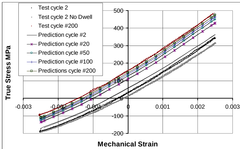
Figure 15. Predicted stress-strain curve against test data for out of phase thermal mechanical fatigue (OP TMF) test up to 0.25% strain range along (001) crystallographic direction at the temperature range from 427 C to 1038 C with hot dwell of 30 minutes
