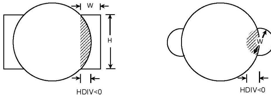
Figure 17. Geometry Definition for Conformal and Semi-Submerged Inlets
