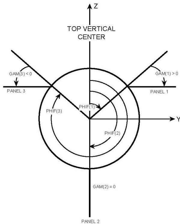
Figure 9. Fin Numbering and Orientation
