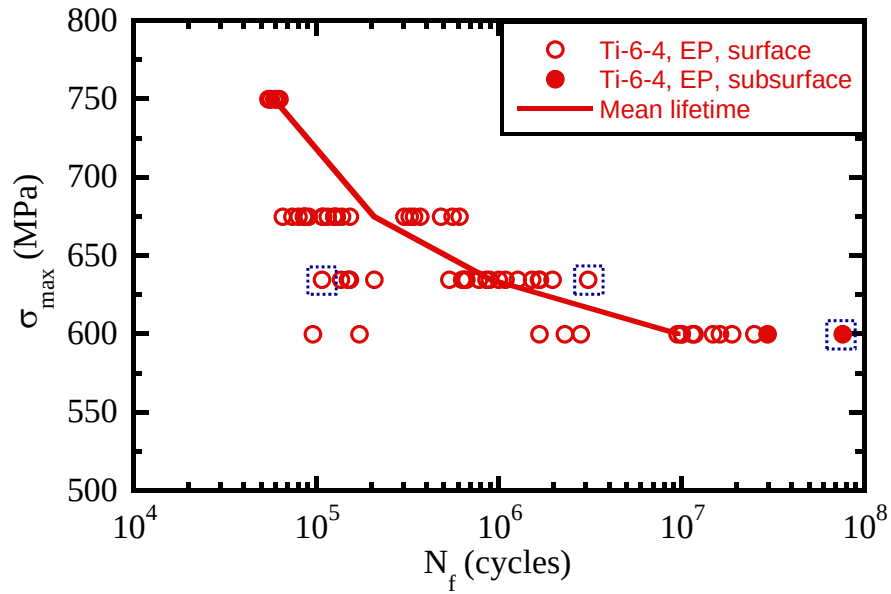
Fig. 2: Fatigue variability behavior of Ti-6-4. The dashed squares indicate the specimens that were selected for characterization of the crack initiation site.
