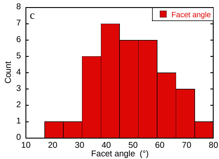
Fig. 7: Crack-initiation in the subsurface crack-initiation specimen tested at 600 MPa with the lifetime of 76,110,019 cycles; (a) the crack-initiation region, (b) facets near the crack origin, and (c) distribution in spatial angle of facets identified in (b).
