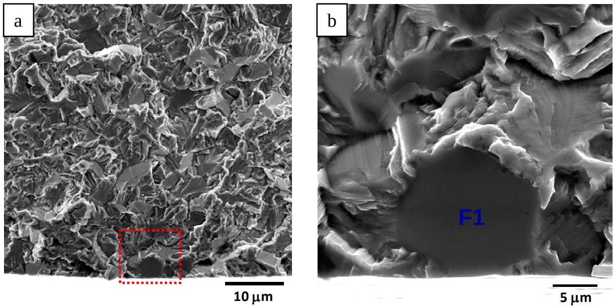
Fig. 3: Crack-initiation in the life-limiting specimen tested at 630 MPa with the lifetime of 106,935 cycles; (a) the crack-initiation region and (b) the suggested crack-initiation facet.
