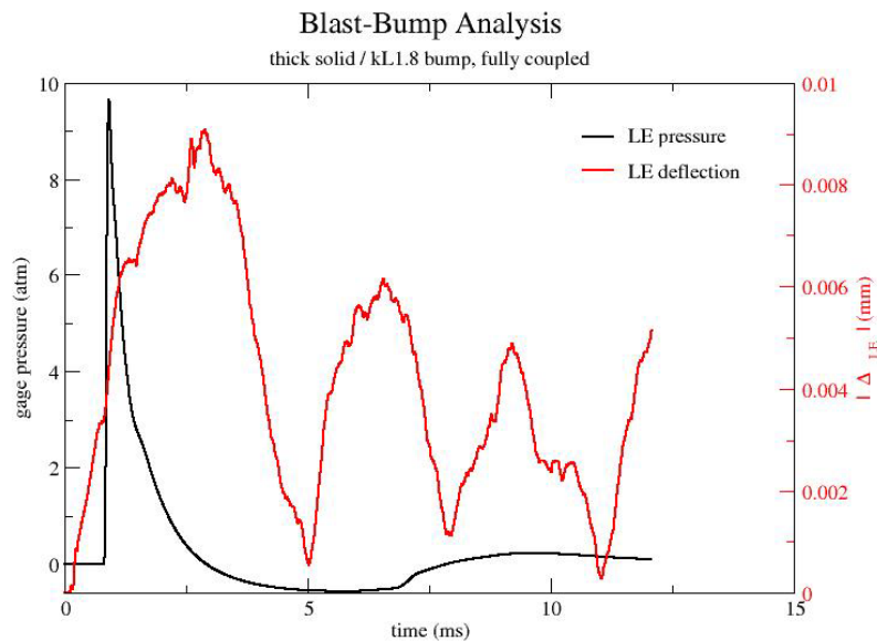
“Thick Solid” (L/H=2) localized response
