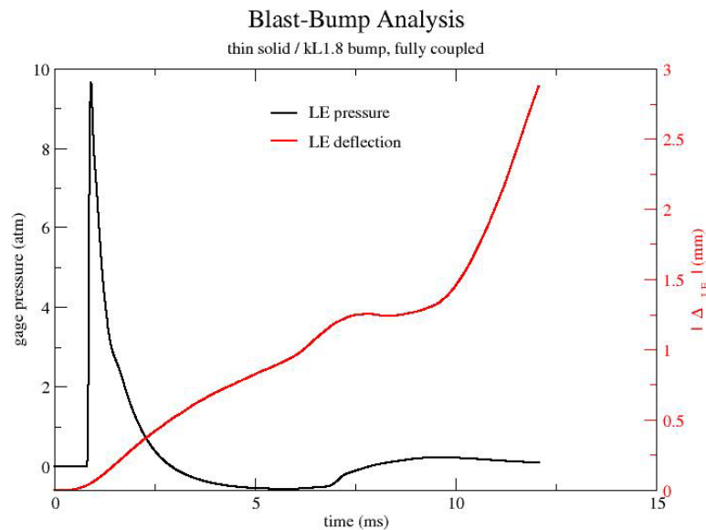
“Thin Solid” (L/H=50) global response
