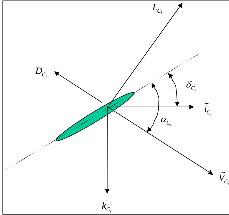
Figure 2. Canard aerodynamic model force diagram.
