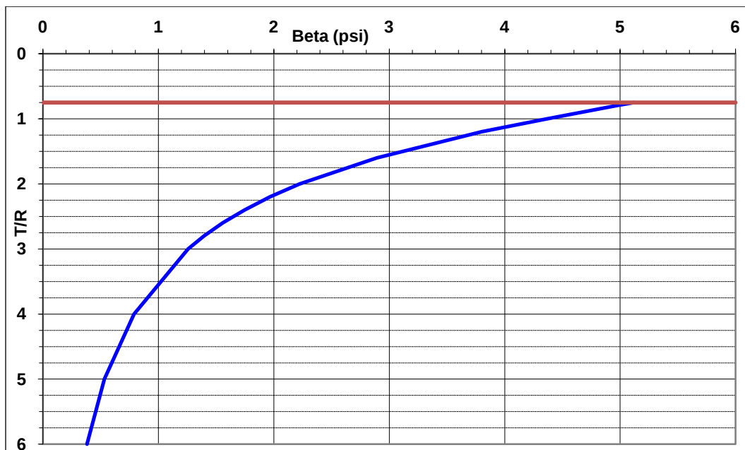
Figure 5. Design chart for base layer ( t_b/R = 0.75 ).
